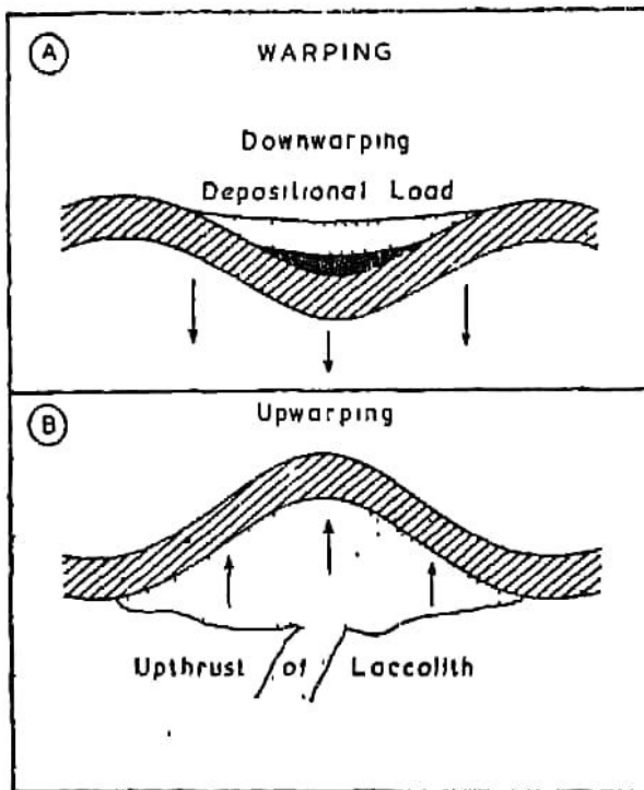
Fig. 49. Downwarping and Upwarping
