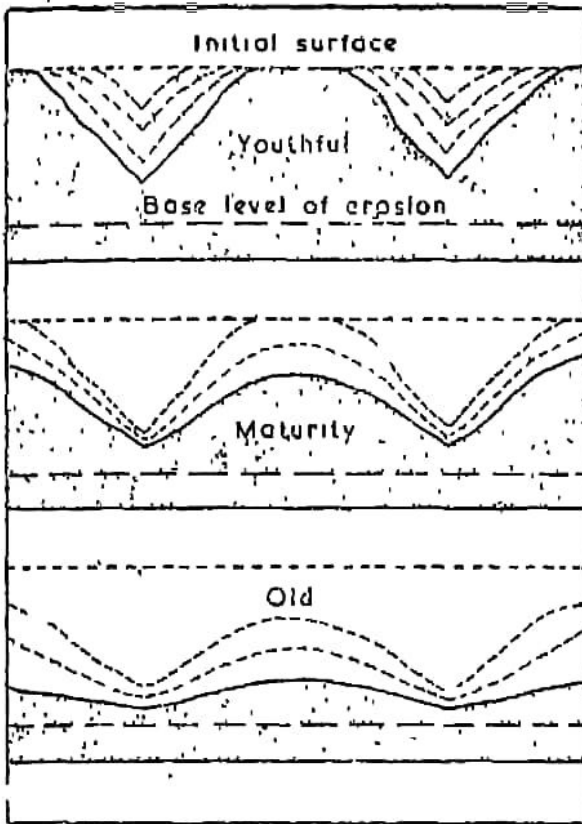
Fig. 26. Cycle of Erosion
