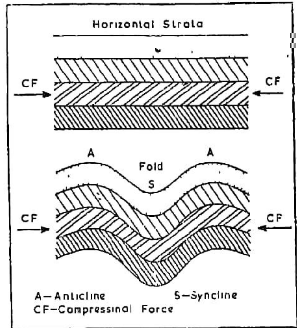
Fig. 45. Horizontal Strata and Compressional Force
