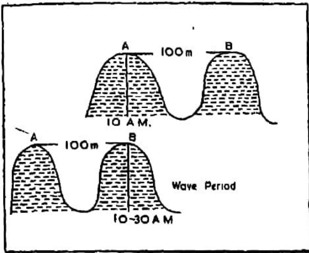
Fig. 106. Wave Velocity
