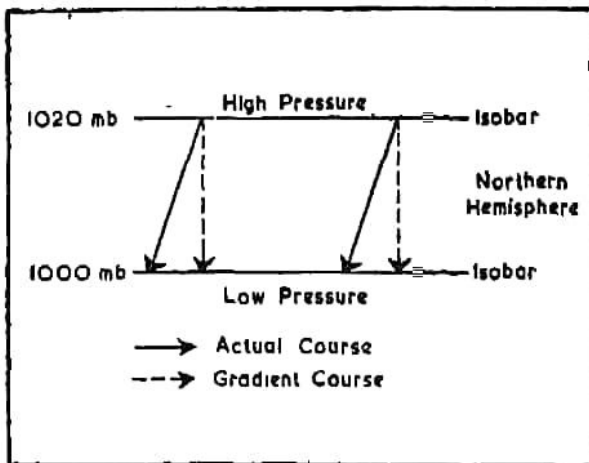
Fig. 69. Relation of Winds to Pressure
