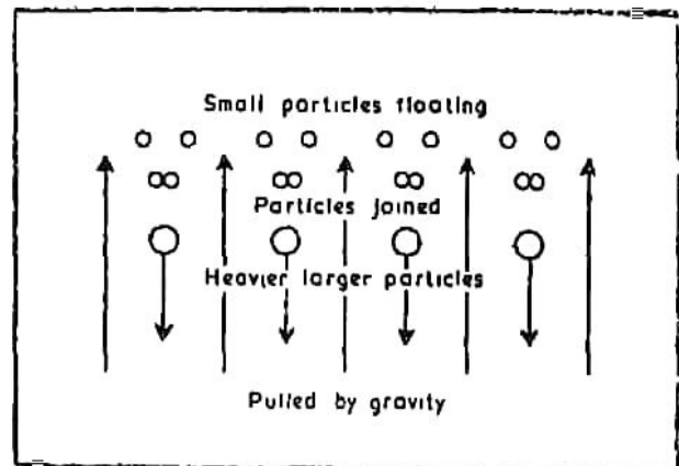
Fig. 79. The Mechanism of Falling of Rain Drops
