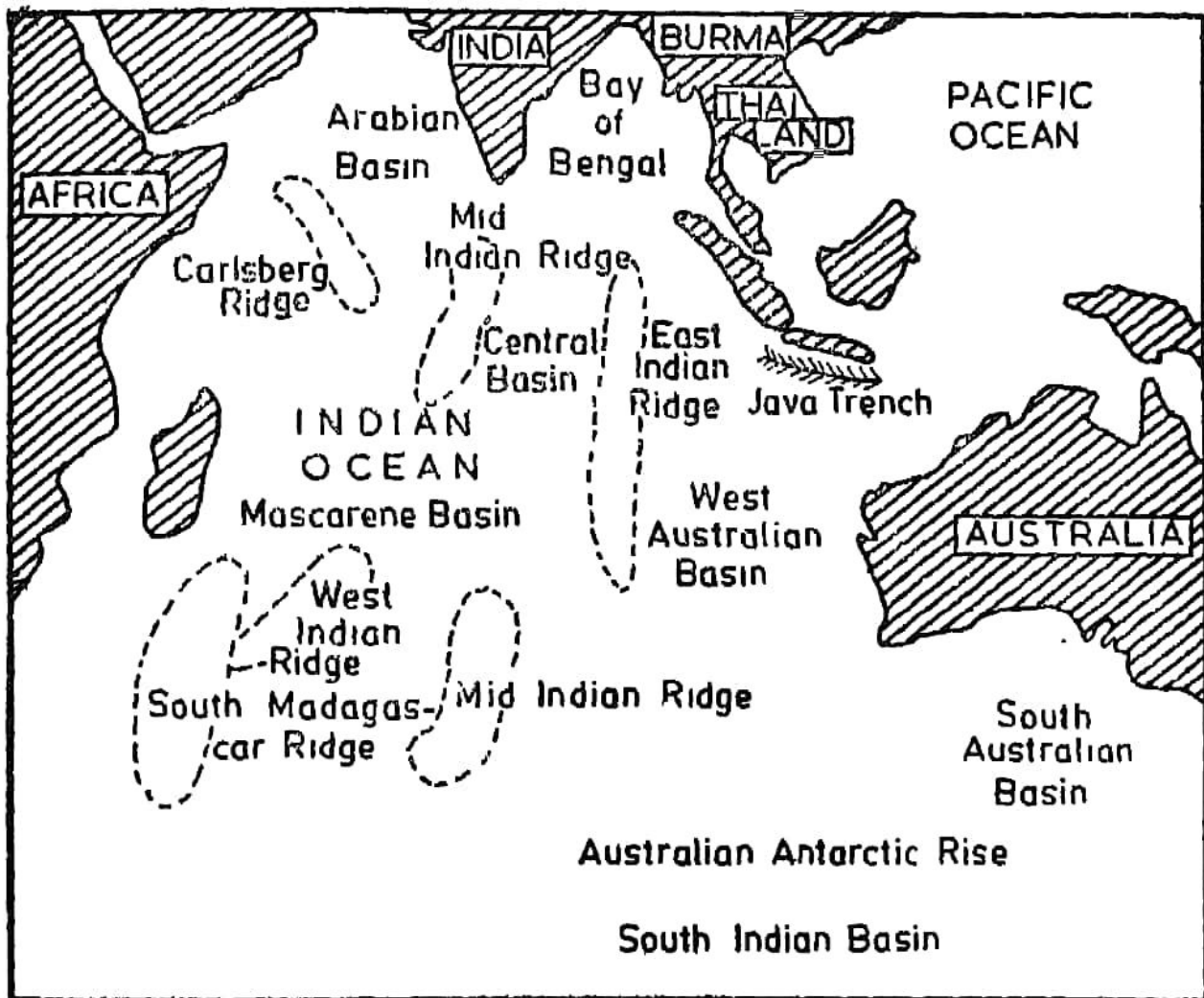
Fig. 102. Indian Ocean Basin Bed Topography
