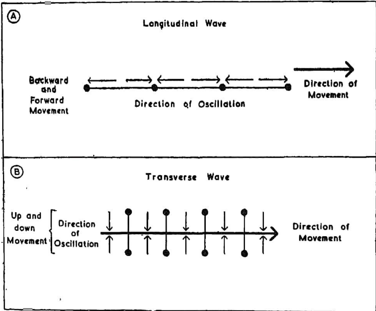
Fig. 5. Longitudinal Wave And Transverse Wave
