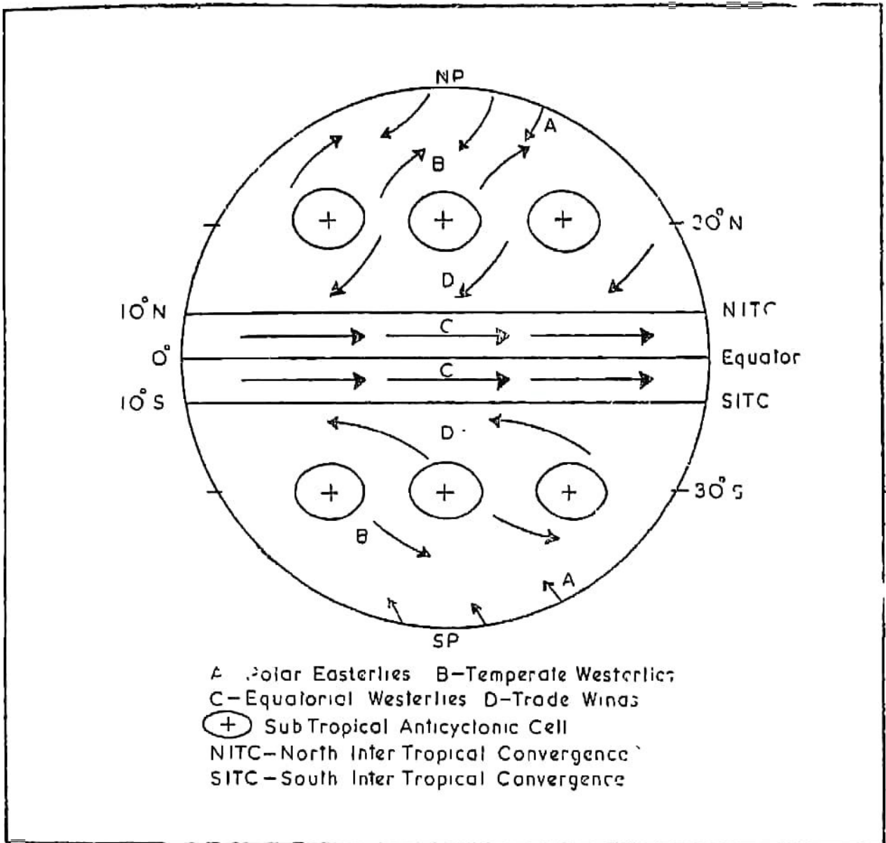
Fig. 71. Origin of Monsoons according to Flohn
