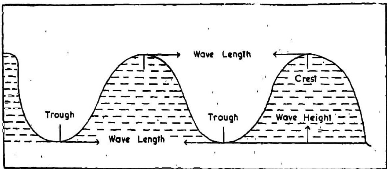
Fig. 105. Wave attributes
