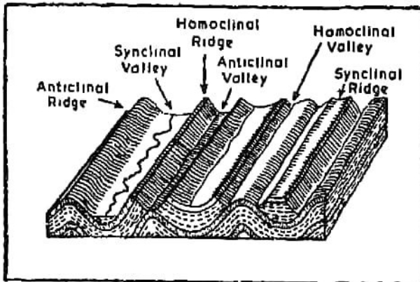
Fig. 46. Valleys in Relation to structural formation
