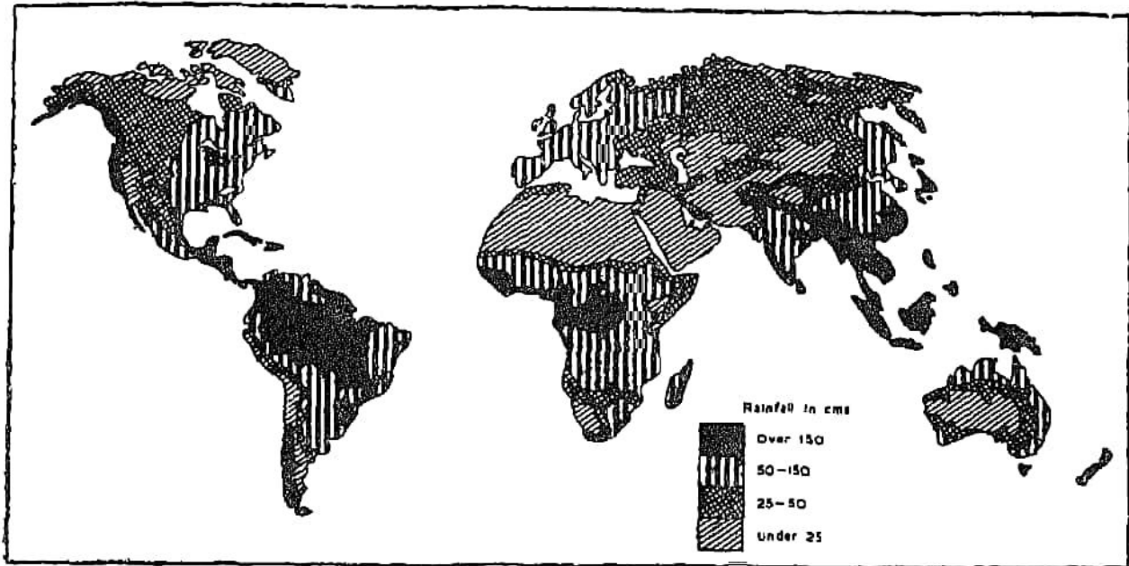
Fig. 80. Distribution of Rainfall
