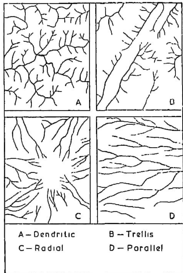
Fig. 27. Drainage Patterns
