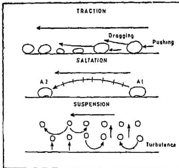
Fig. 25. Traction, saltation, suspension
