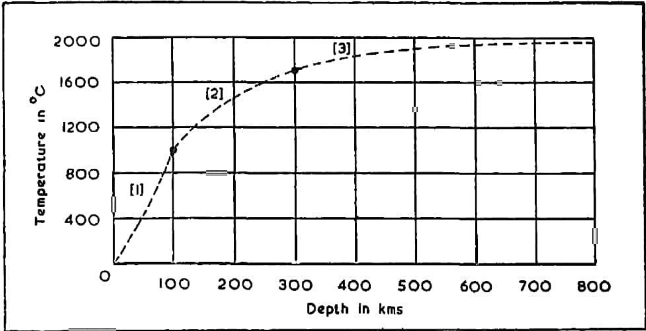
Fig. 12. Variation of temperature with depth
