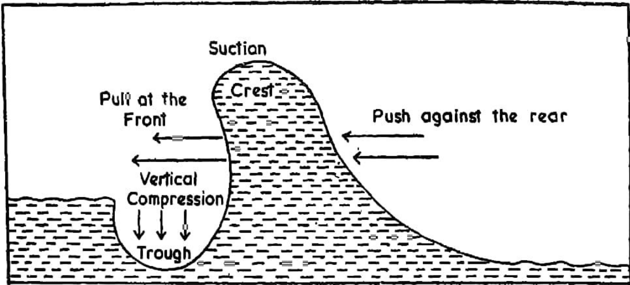
Fig. 104. Formation of Wave
