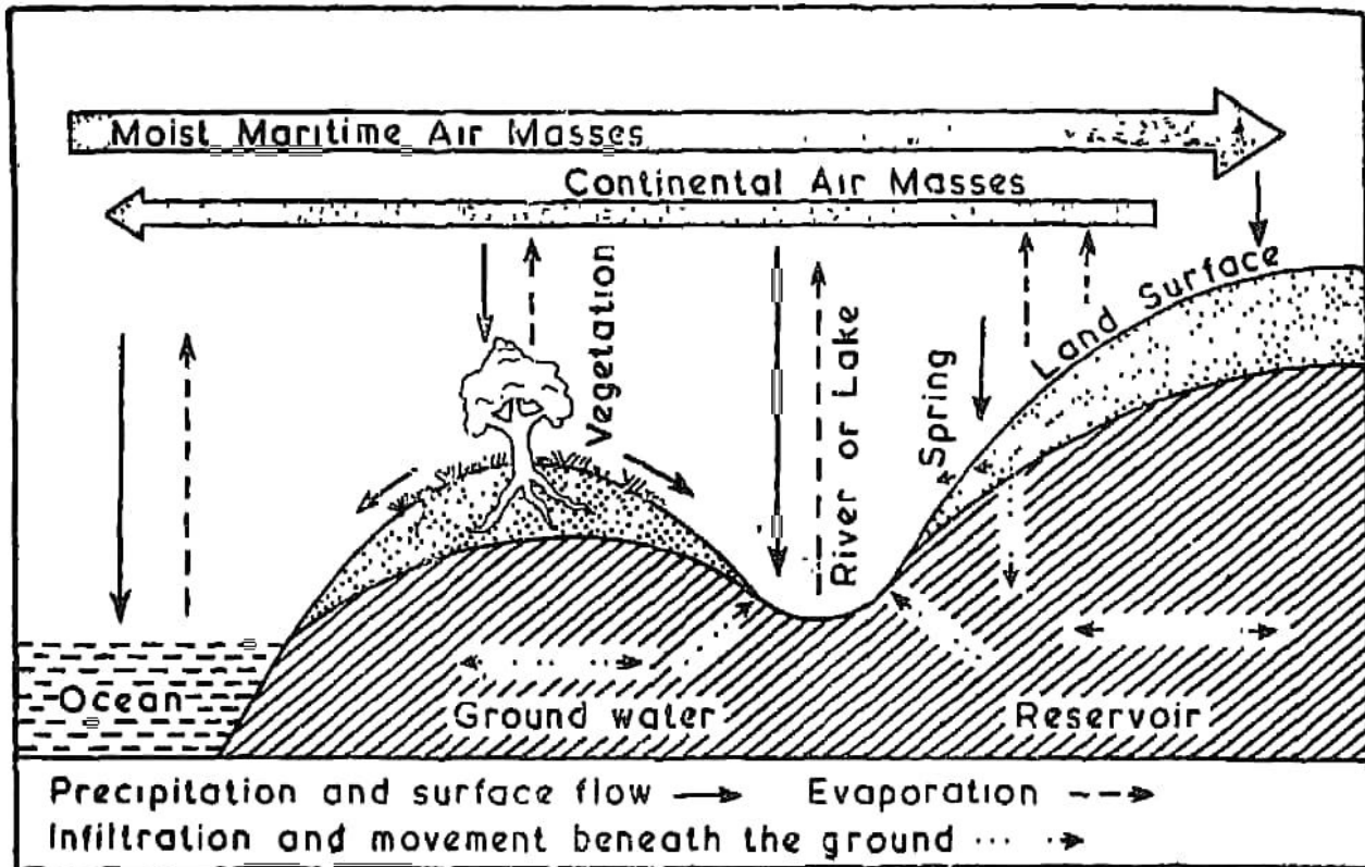
Fig. 83. The Hydrologic Cycle
