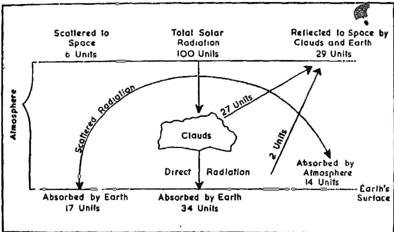
Fig. 60. Heat Budget
