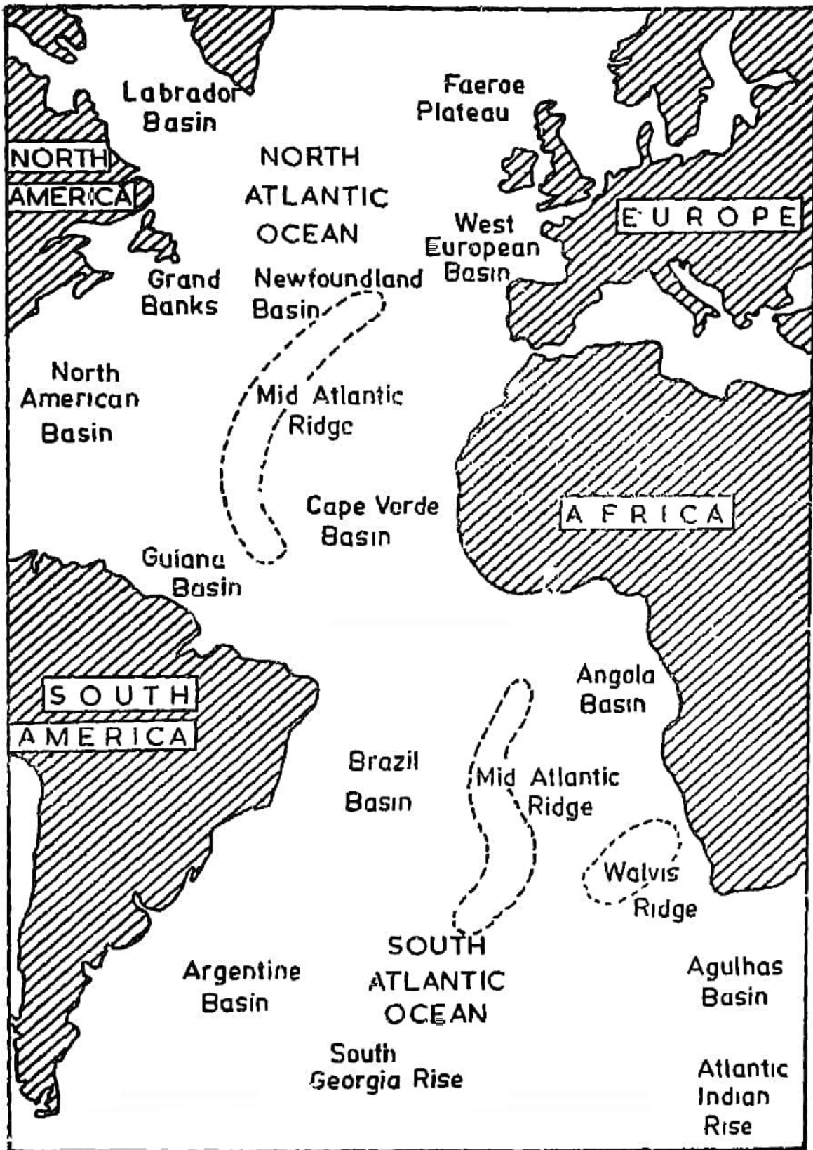
Fig. 101. Atlantic Ocean Basin Bed Topography
