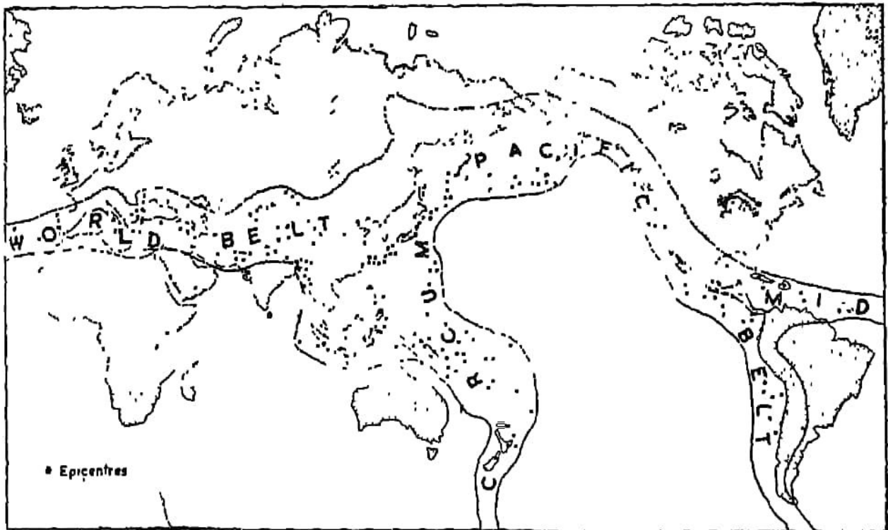
Fig. 55. Earthquake Belts of the World
