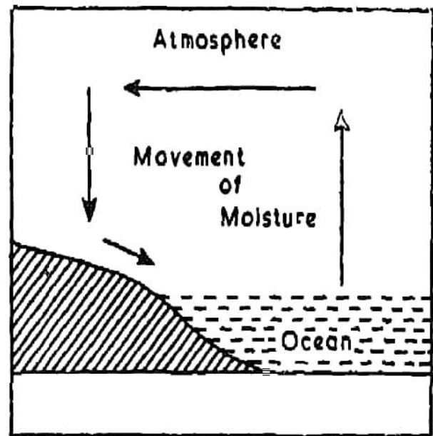
Fig. 82. Simple Hydrologic Cycle ture, e.g., the moisture that goes into the atmosphere may be precipitated into water, dew, snow, ice, frost and the like. Similarly, water collects in various forms. The water that comes down from the atmosphere may enter a river, a lake,
