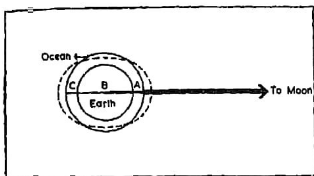
Fig. 109. Formation of Tide
