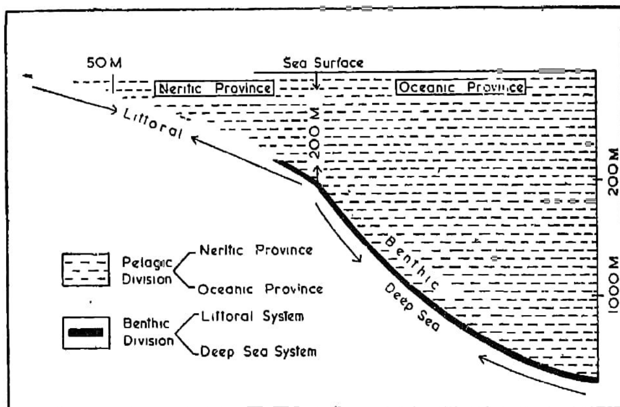
Fig. 111. The Principal Division of Marine Environment.
