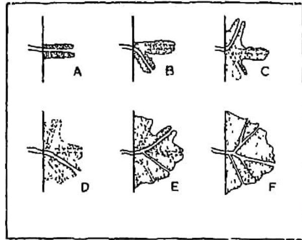
Fig. 37. Stages in formation of a Simple Delta
