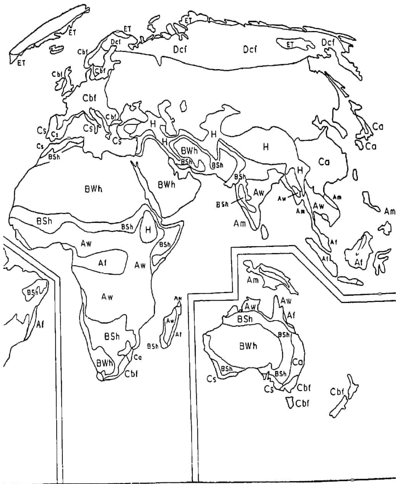
Fig. 81. Types of Climate
