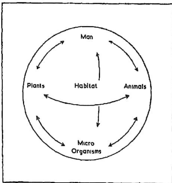
Fig. 3. Interacting Elements of Biosphere
