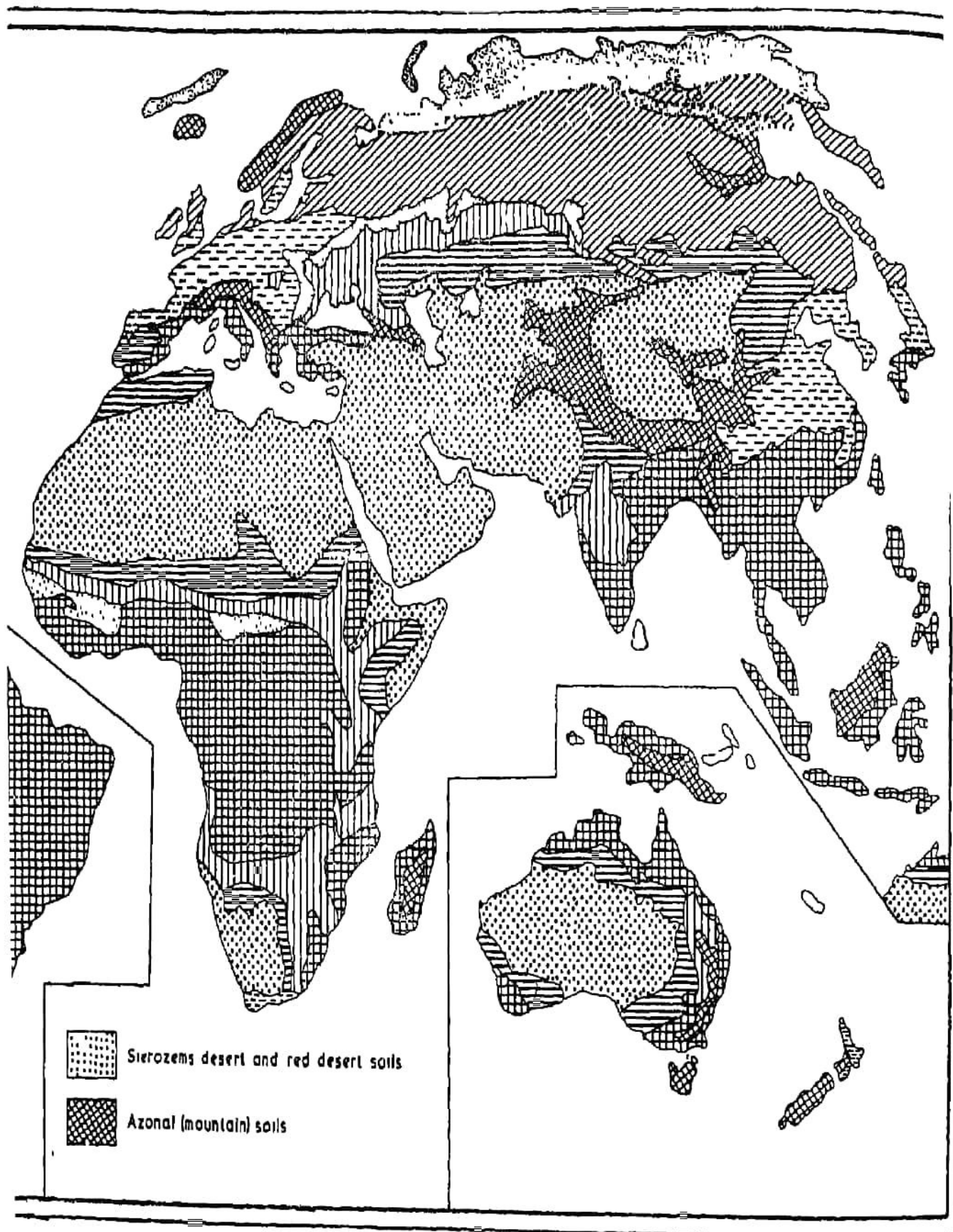
Fig. 23. Main Soil Types
