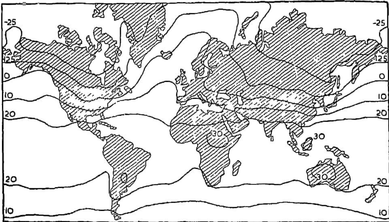
Fig. 63. January Isotherms
