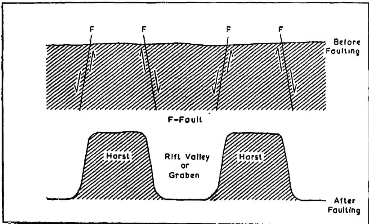
Fig. 48. Formation of Horst and Graben
