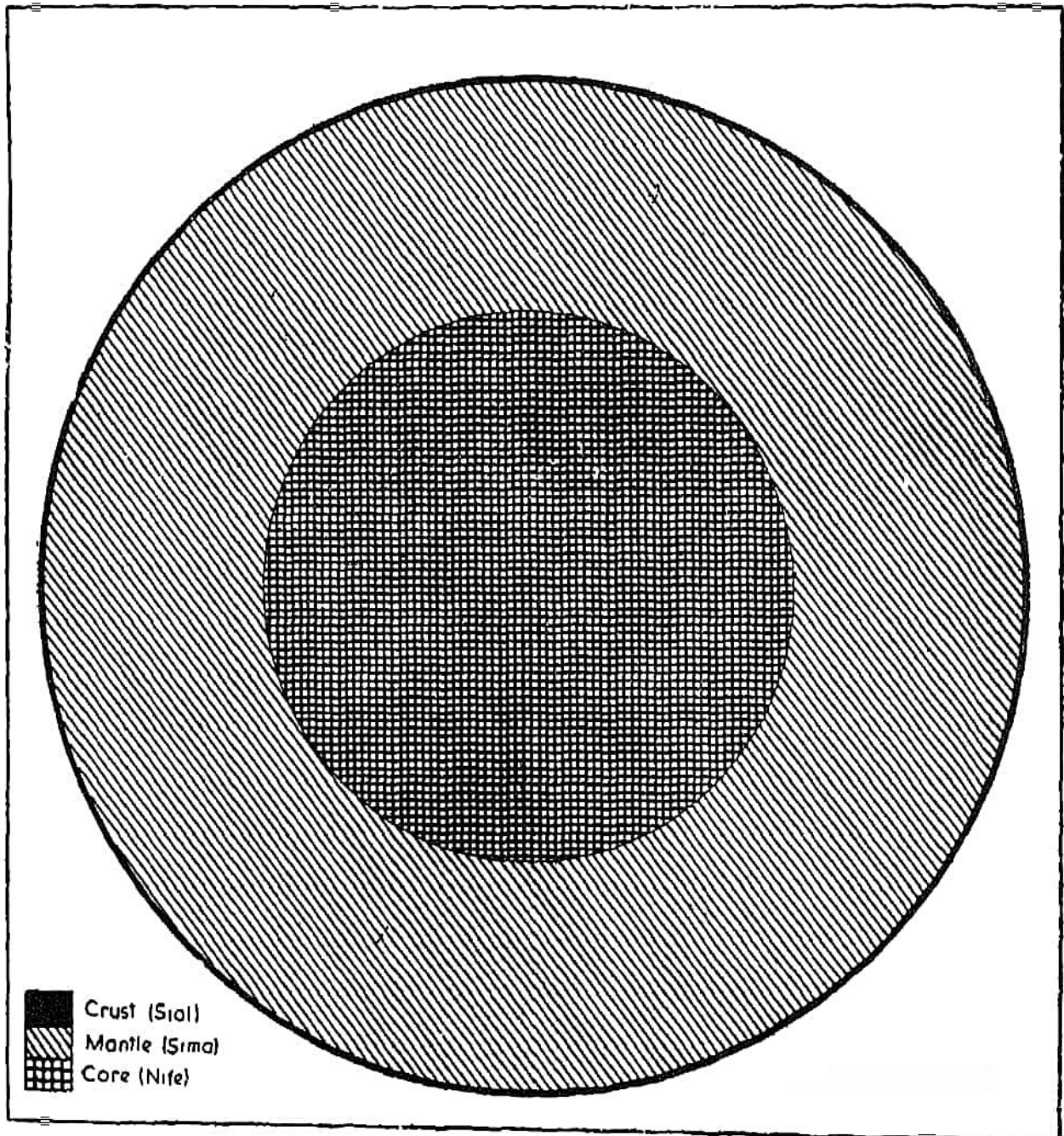
Fig. 10. The main layers of earth's body
