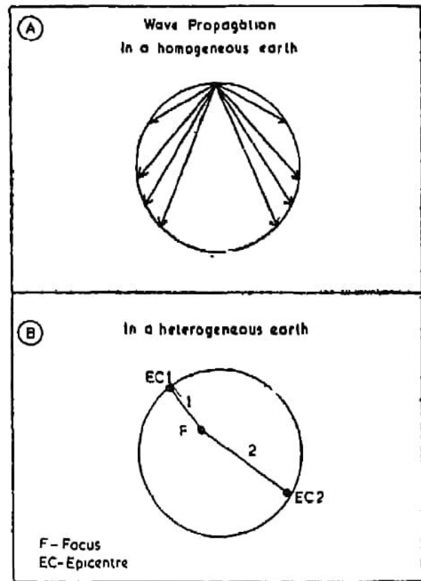
Fig. 6. Wave Propagation
