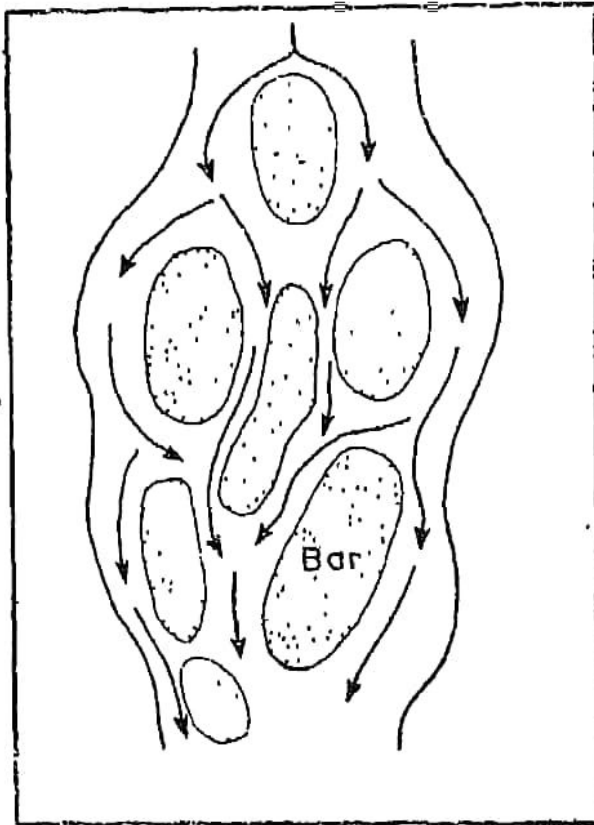
Fig. 36. Braided Stream
