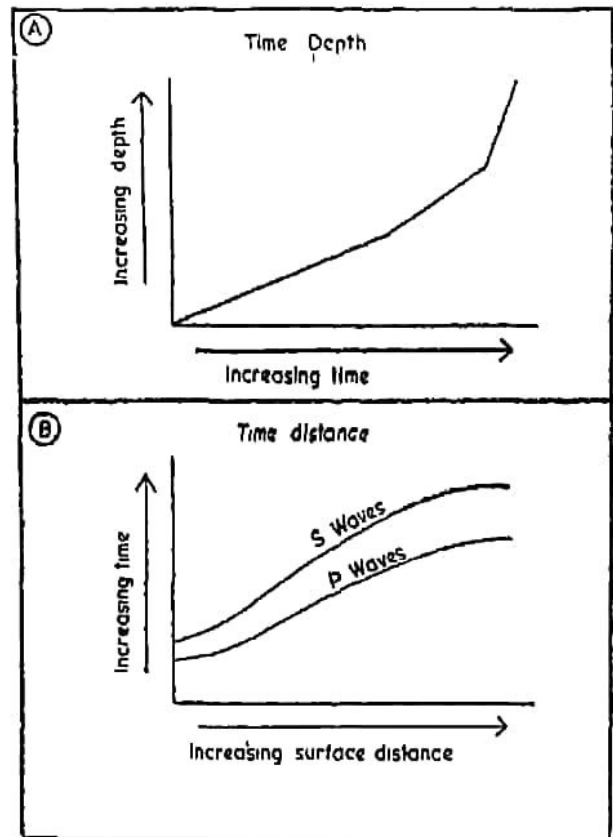
Fig. 8. Wave travel curves
