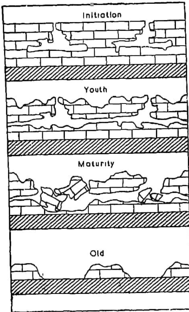
Fig. 96—The Cycle of Karst Erosion
