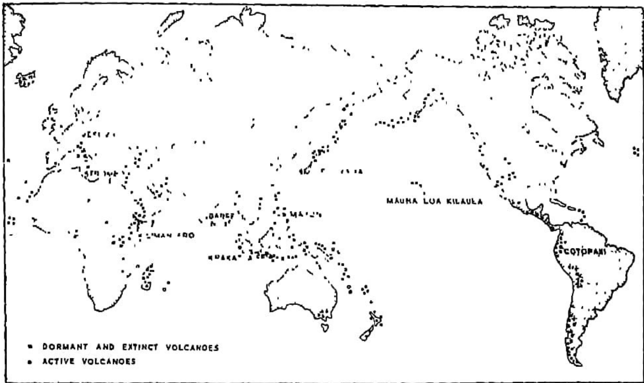
Fig. 54. The Distribution of Volcanoes
