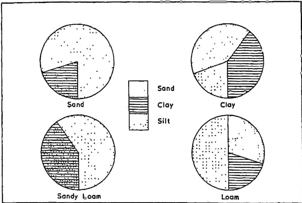
Fig. 22. Main Textural types of soil
