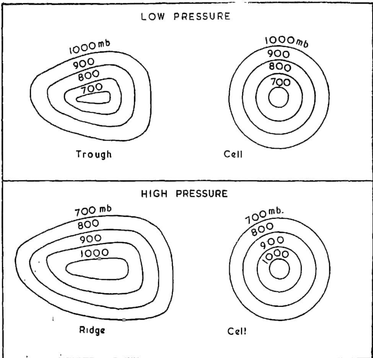
Fig. 65. Low Pressure and High Pressure
