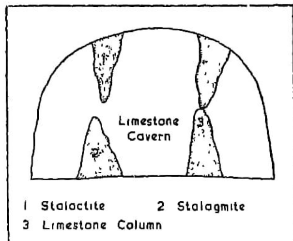
Fig. 95. Stalactite, Stalagmite and Limestone Column.
