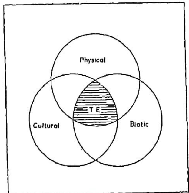
Fig. 4. Total Environment
