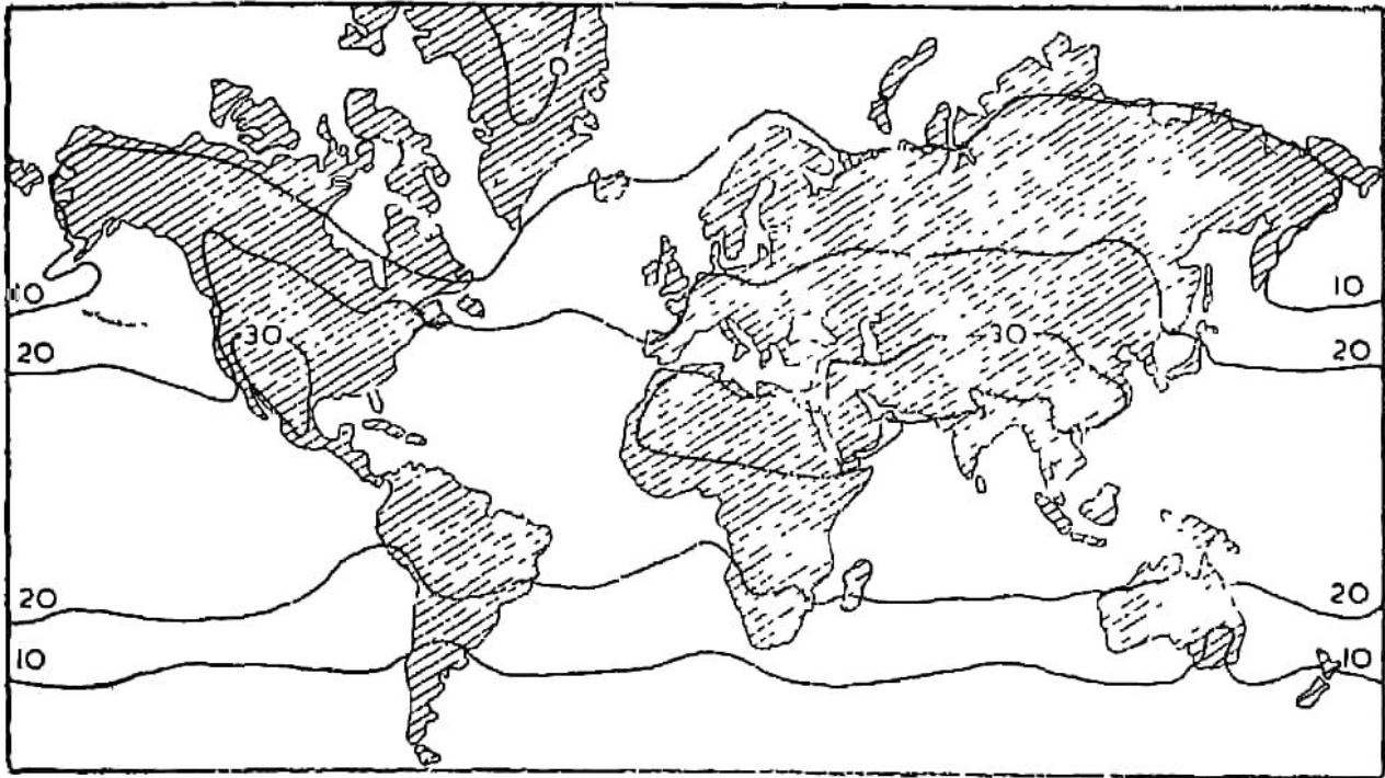
Fig. 64. July Isotherms
