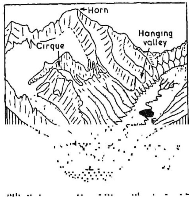
Fig. 41. Glacial Features
