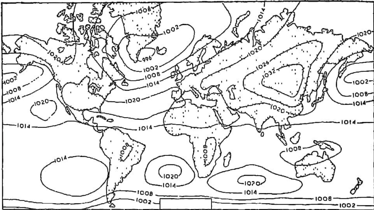
Fig. 66. January Isobars
