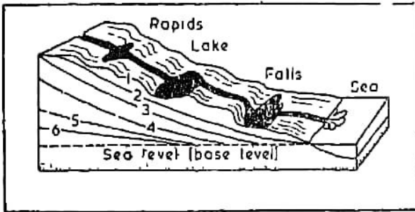
Fig. 30. Gradation of a Stream
