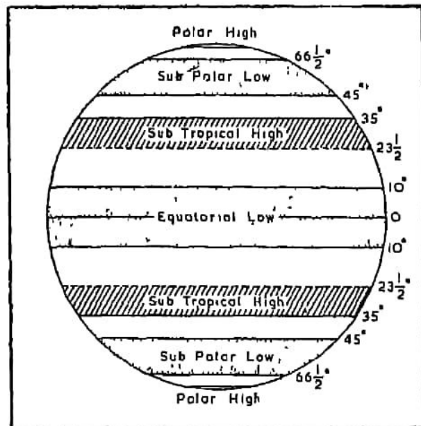
Fig. 68. Pressure Belts
