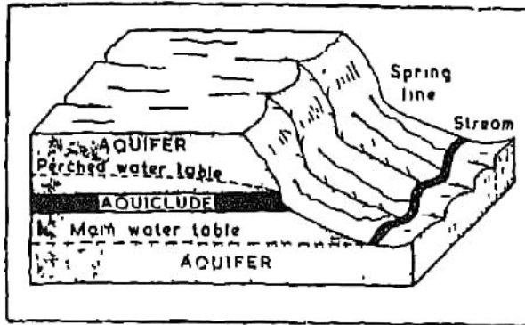
Fig. 90. Rock Structure and Springs
