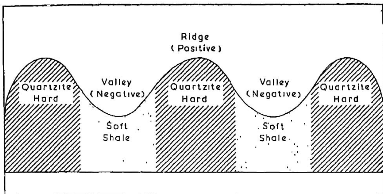
Fig. 19. Rock Hardness and Relief Features
