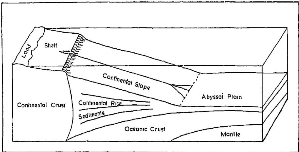
Fig. 97. Continental and Oceanic Crust
