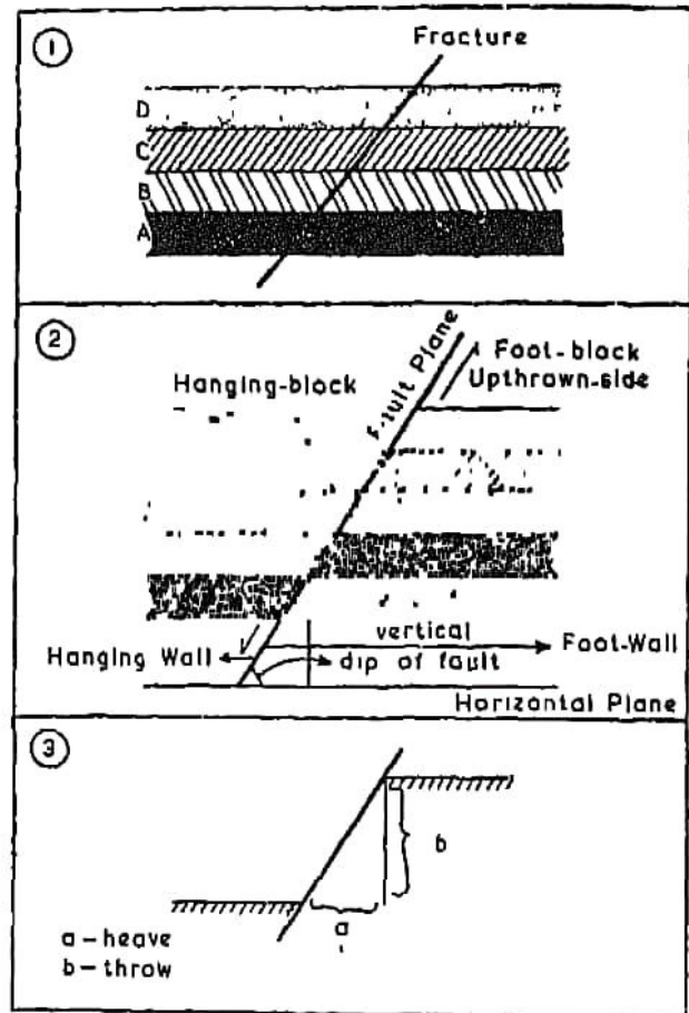
Fig. 47. Fracture and Fault Plane
