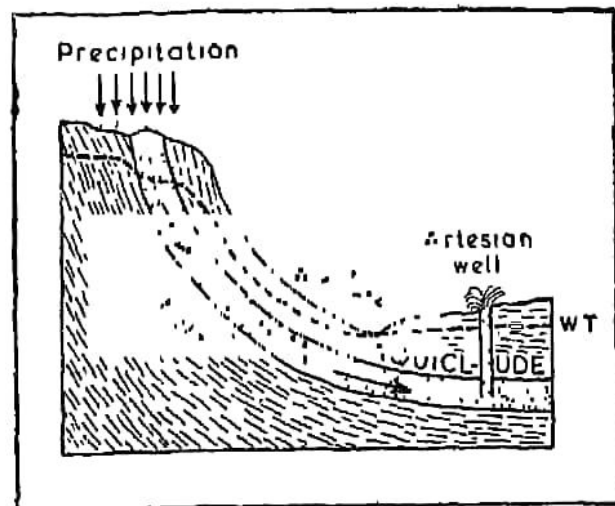
Fig. 93. Geological conditions for Artesian flow
