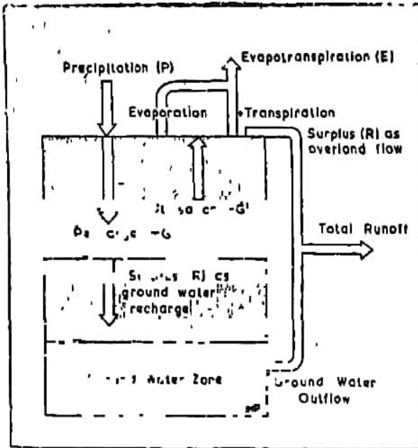
Fig. 85. Soil Water Balance
