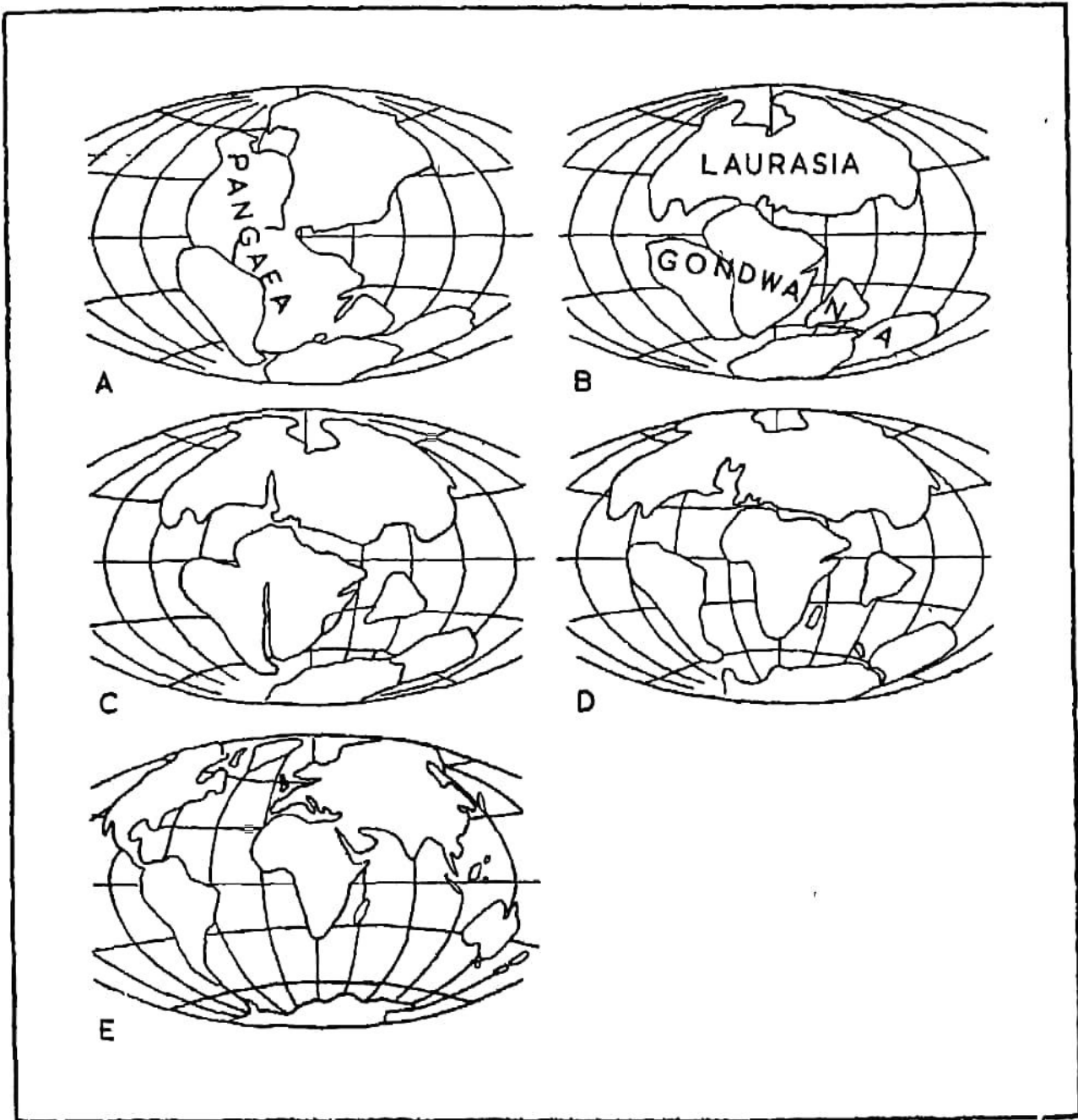
Fig. 52. Continental Drift
