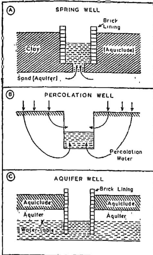
Fig. 92. Spring well, Percolation well and Aquifer well
