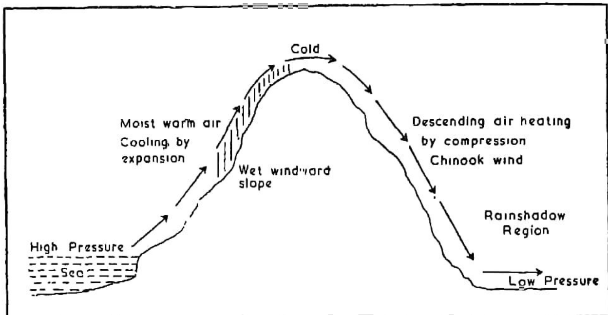
Fig. 72. Formation of Foehn and Chinook
