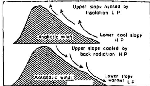
Fig. 74. Anabatic Winds and Katabatic Winds
