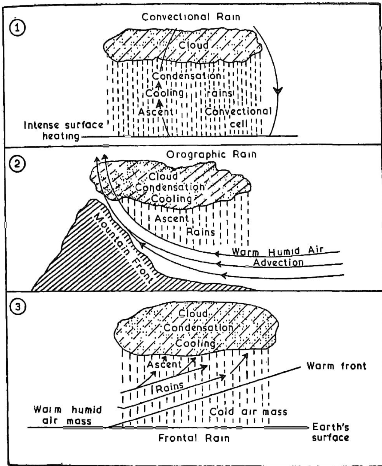
Fig. 78. Convective Rain, Orographic Rain and Frontal Rain
