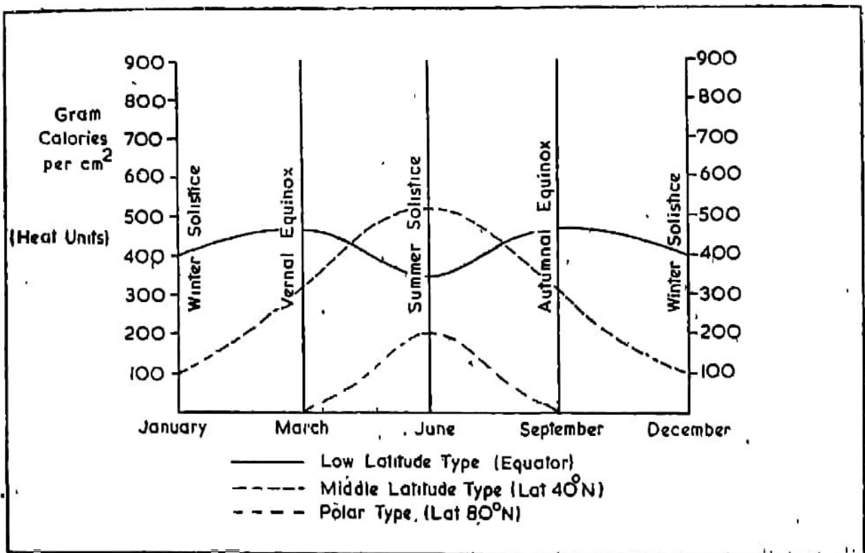
Fig. 59. March of Insolation
