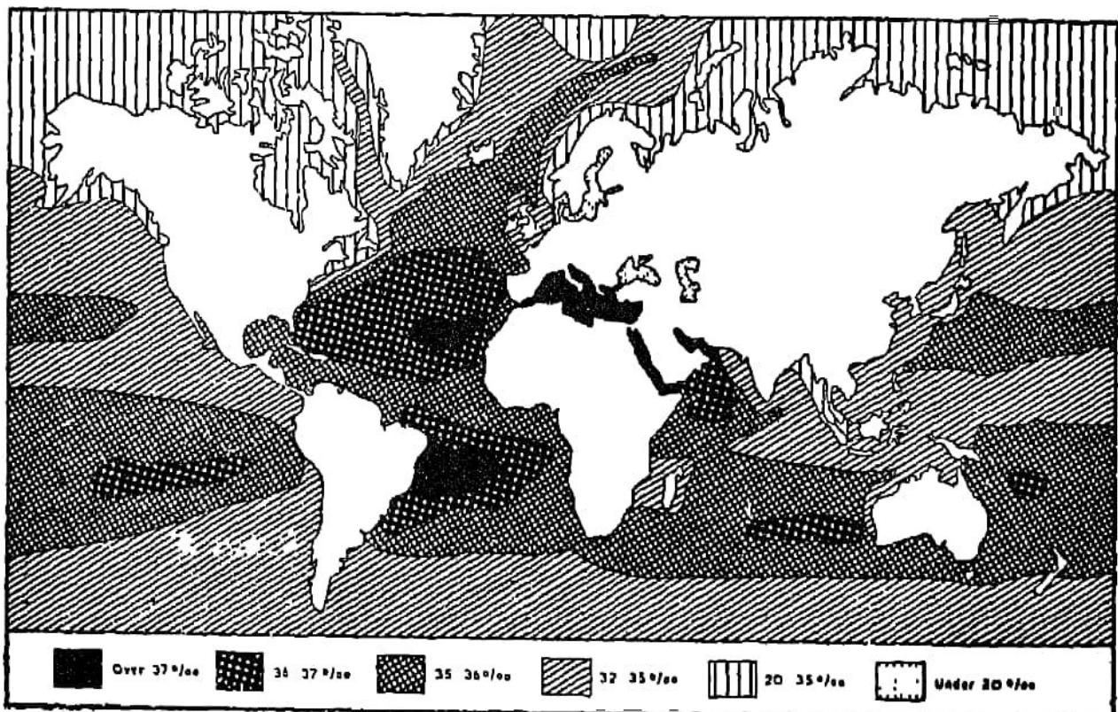
Fig. 103. Distribution of Salinity
