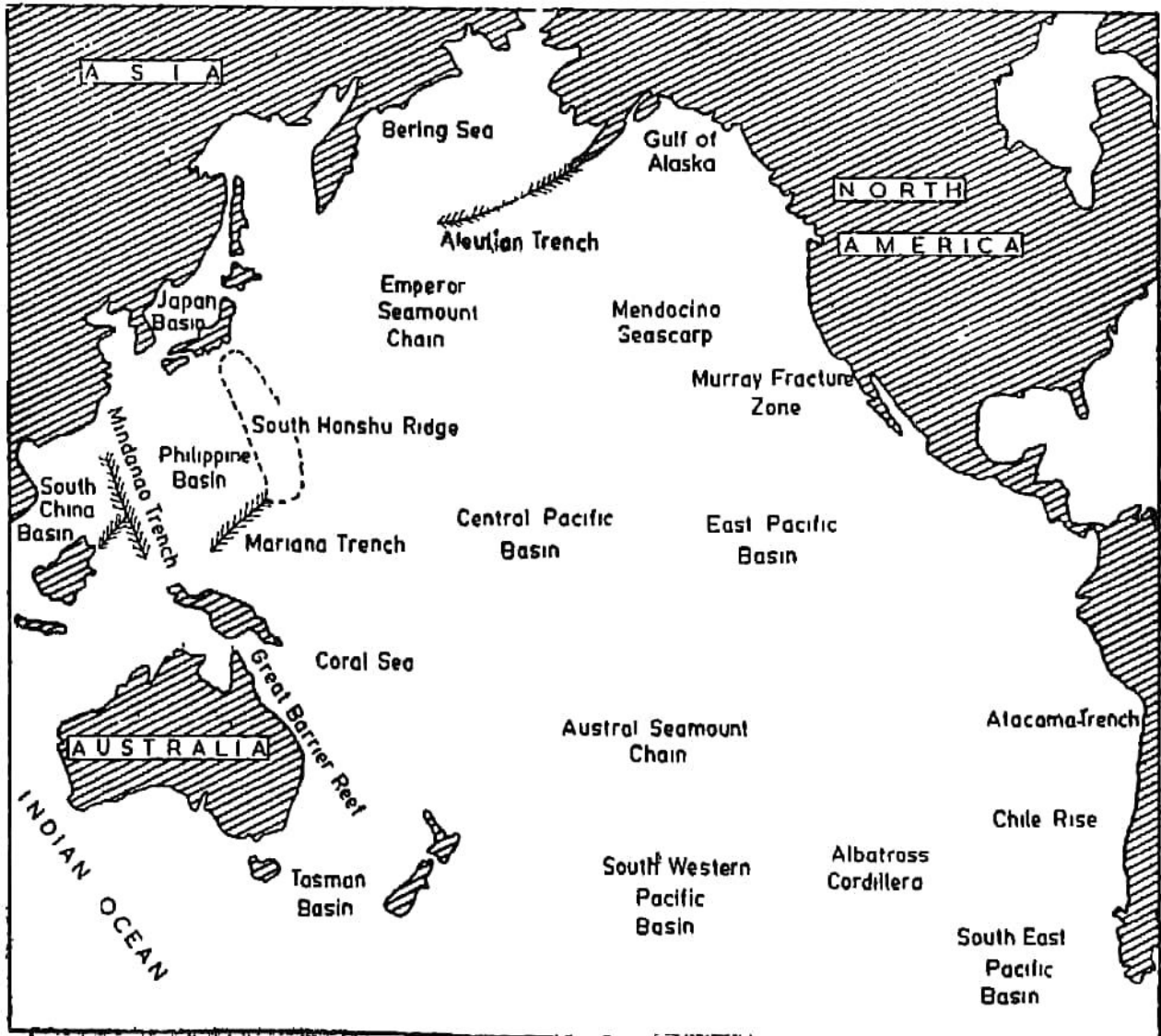
Fig. 100. Pacific Ocean Basin Bed Topography
