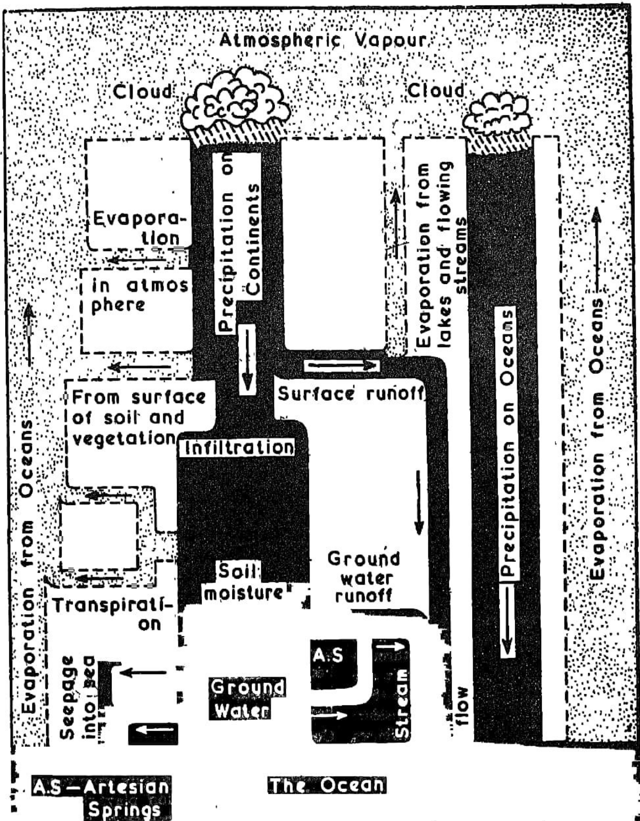
Fig. 84. A Model of Hydrologic Cycle
