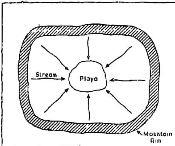
Fig. 38. Intermontane Desert
