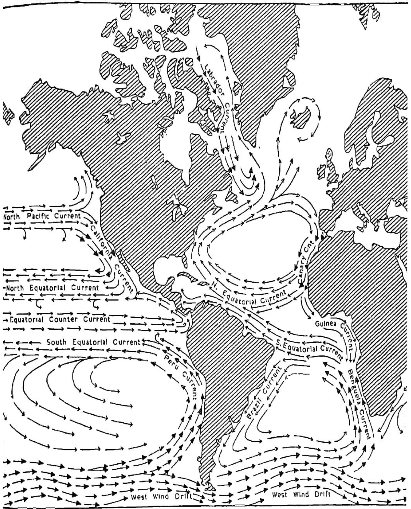
Fig 108. Ocean Currents
