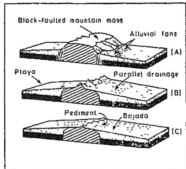
Fig. 40. The Erosional Evolution of a Pediment
