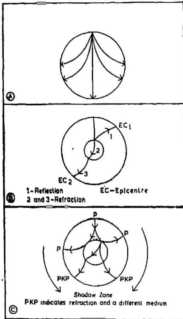
Fig. 7. Paths of Wave in the earth
