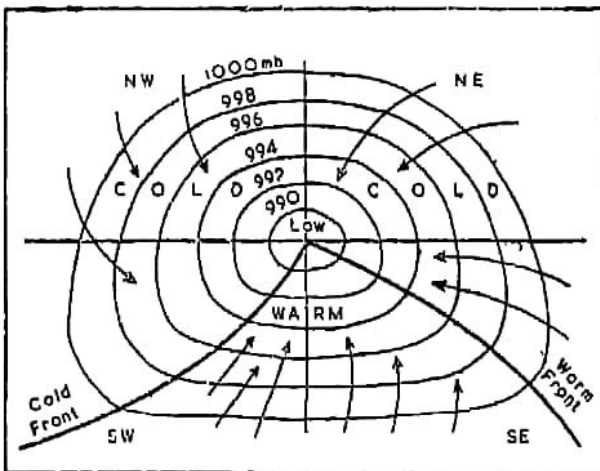
Fig. 76. Cyclone in the Northern Hemisphere
