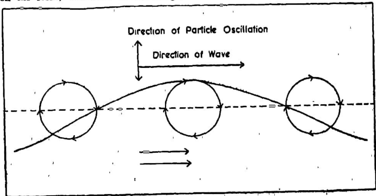
Fig. 107. Transverse Wave
