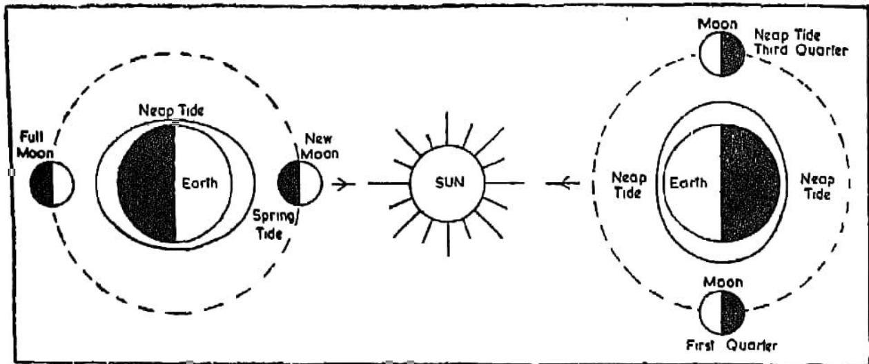
Fig. 110. Formation of Spring and Neap Tides
