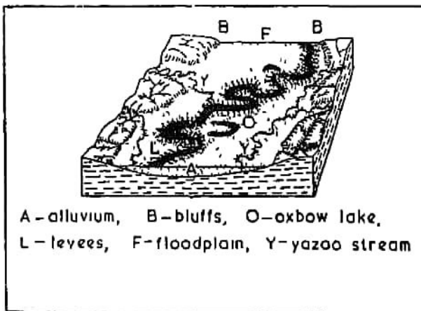
Fig. 31. Landforms of an Alluvial River Flood Plain
