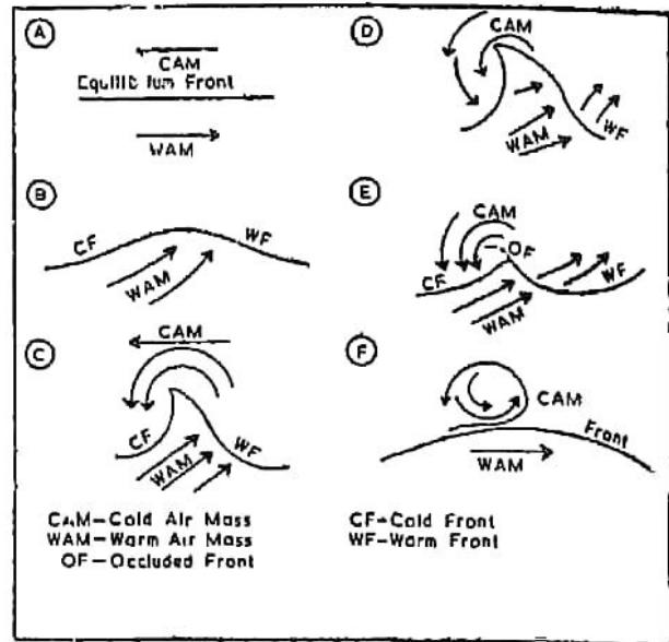
Fig. 77. Cold and Warm Air masses and Fronts
