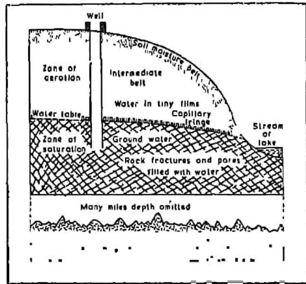
Fig. 86. Zones of Subsurface Water Water Table
