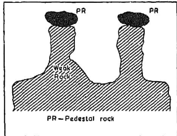
Fig. 39. Pedestal Rock
