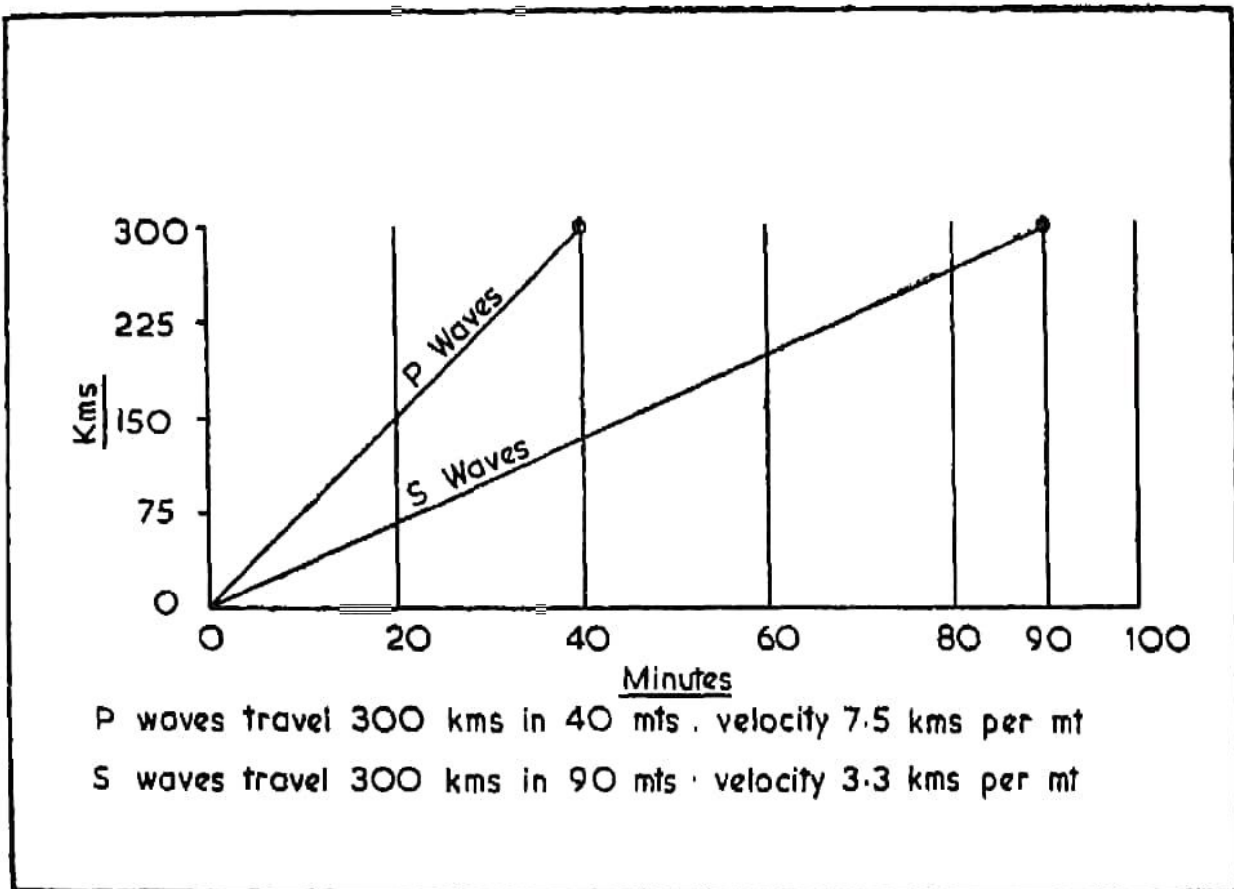
Fig. 9. Wave Propagation Velocity
