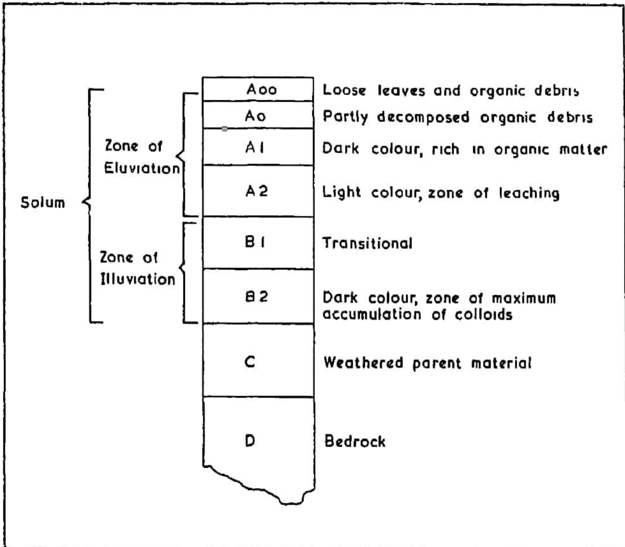
Fig. 21. Generalised Soil Profile
