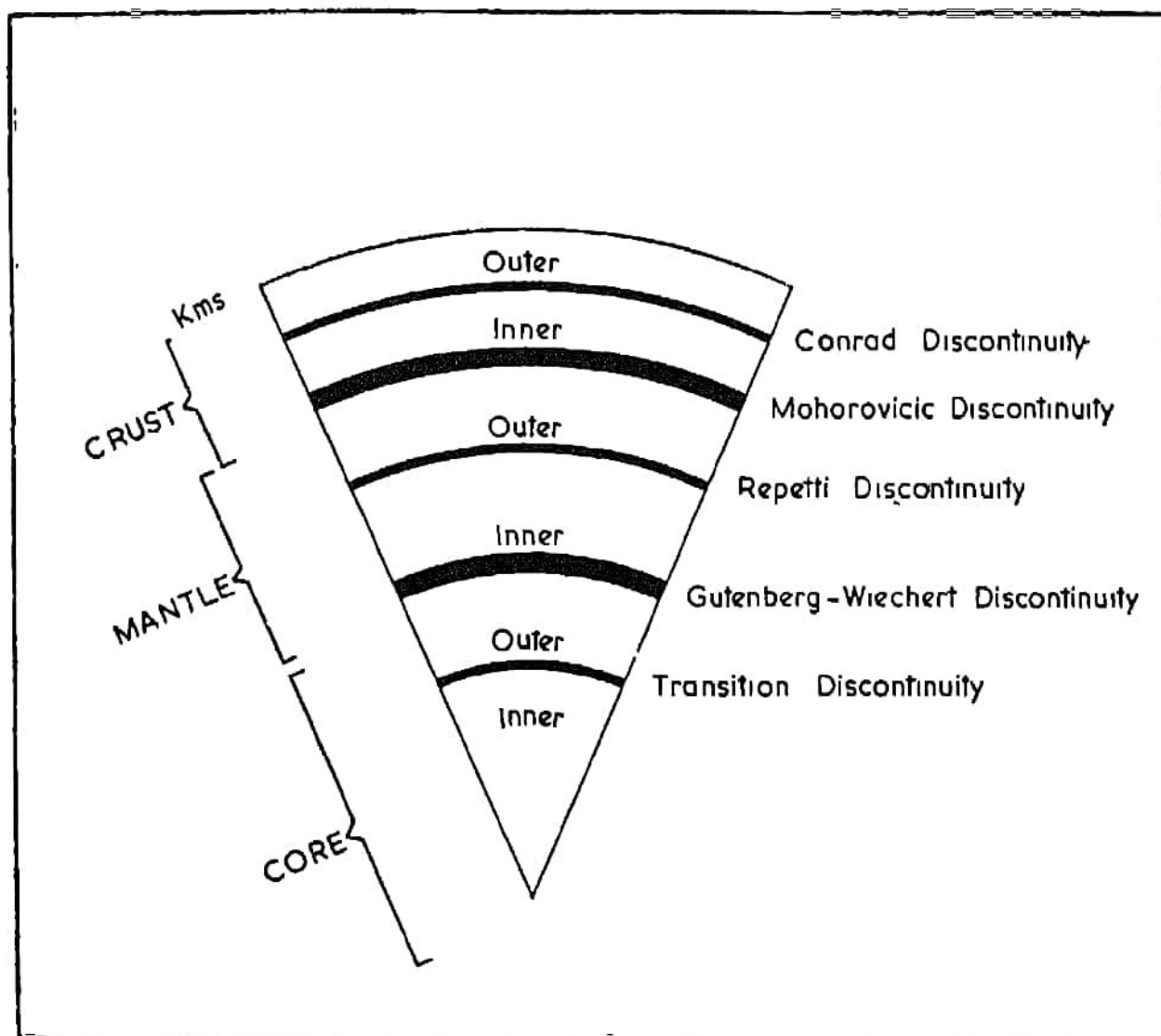
Fig. 11. Model of earth's interior
