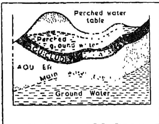
Fig. 88. Perched Ground Water
