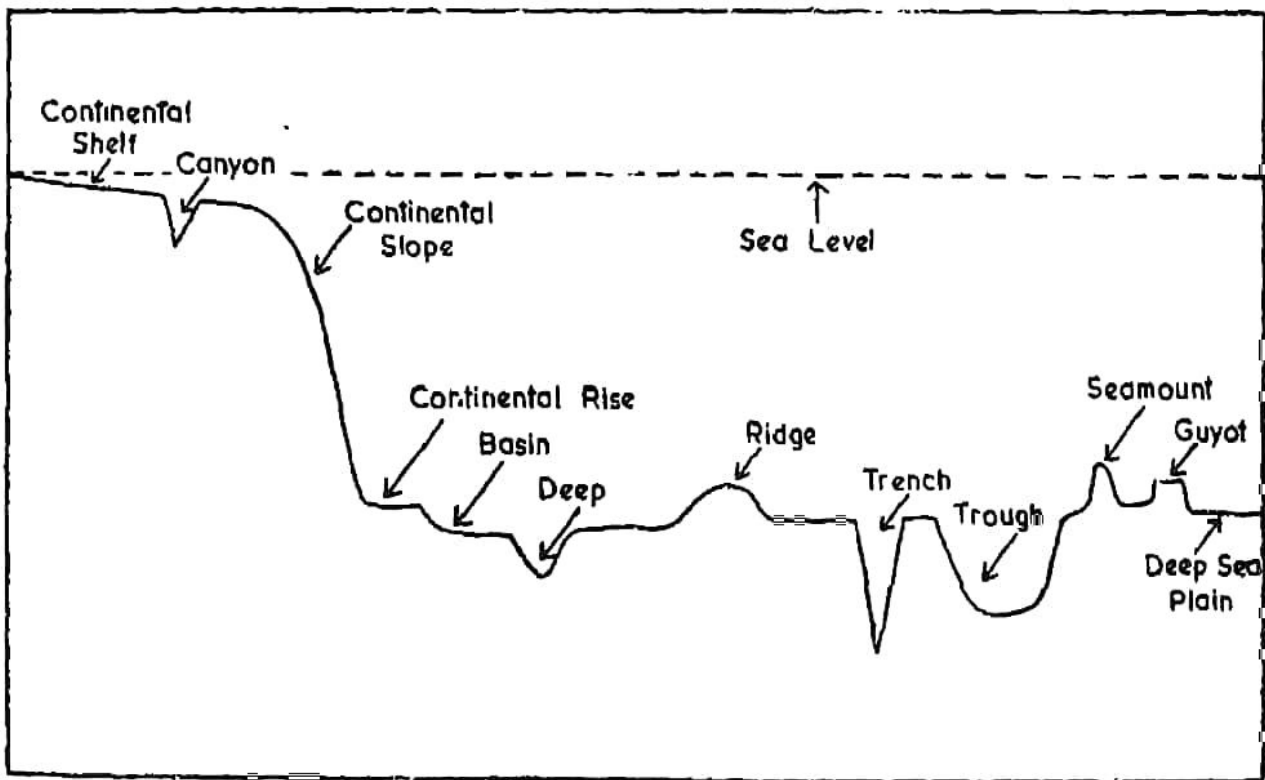
Fig. 98. Topographical Features of the Sea Bottom
