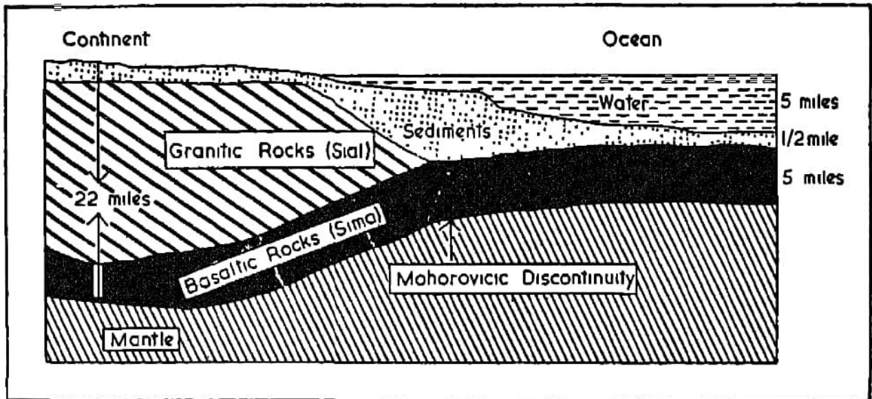
Fig. 13. Profile of the earth's crust
