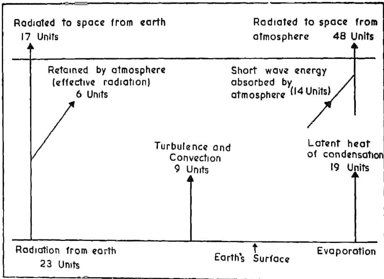
Fig. 61. Terrestrial Radiation
