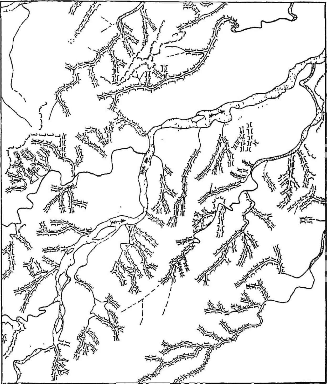
Fig. 20. Clay Topography
