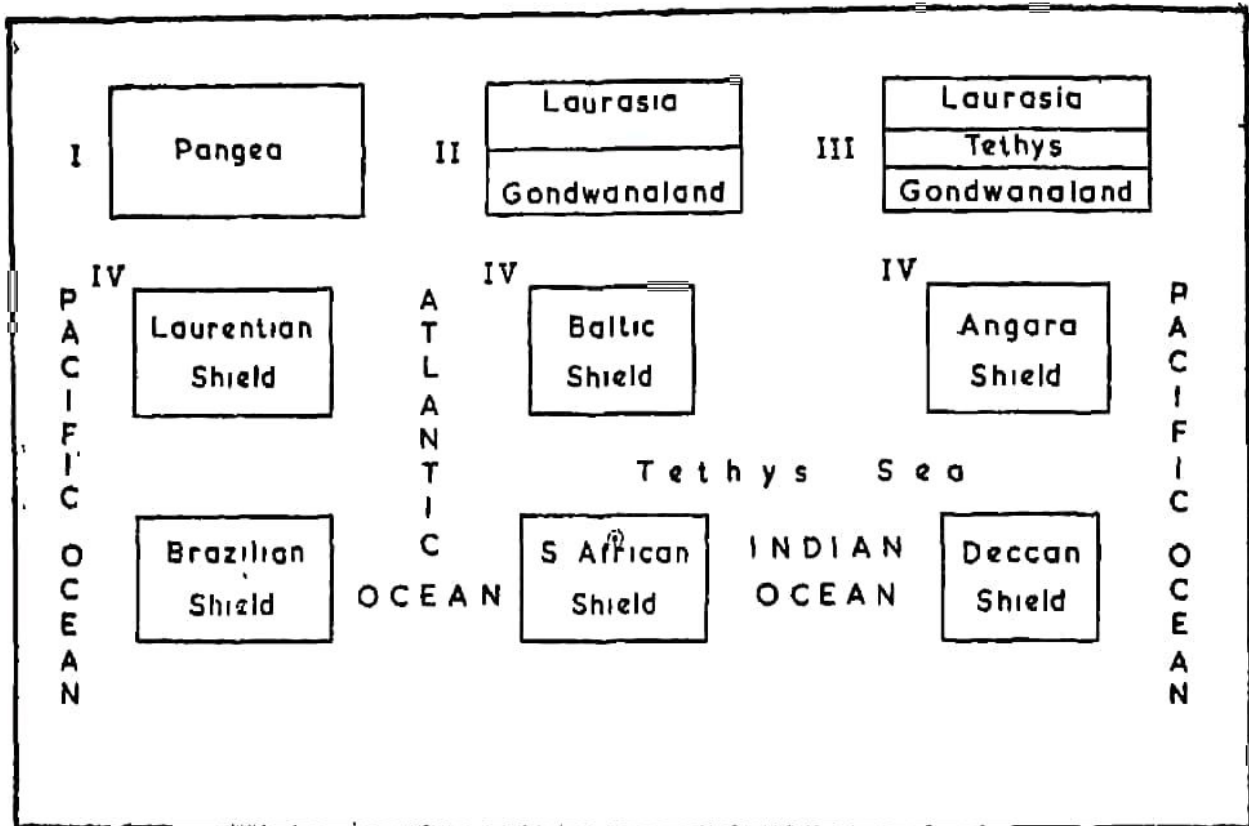
Fig. 51. Sequences in Continental Drift.
