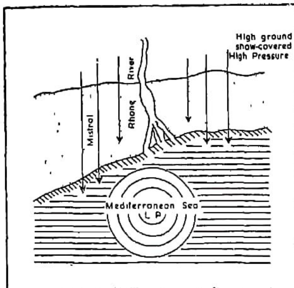
Fig. 73. Formation of Mistral
