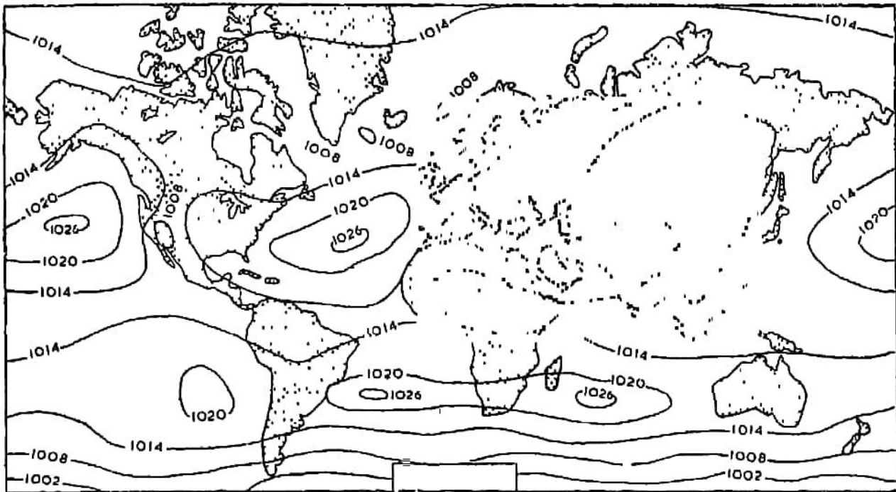
Fig. 67. July Isobars
