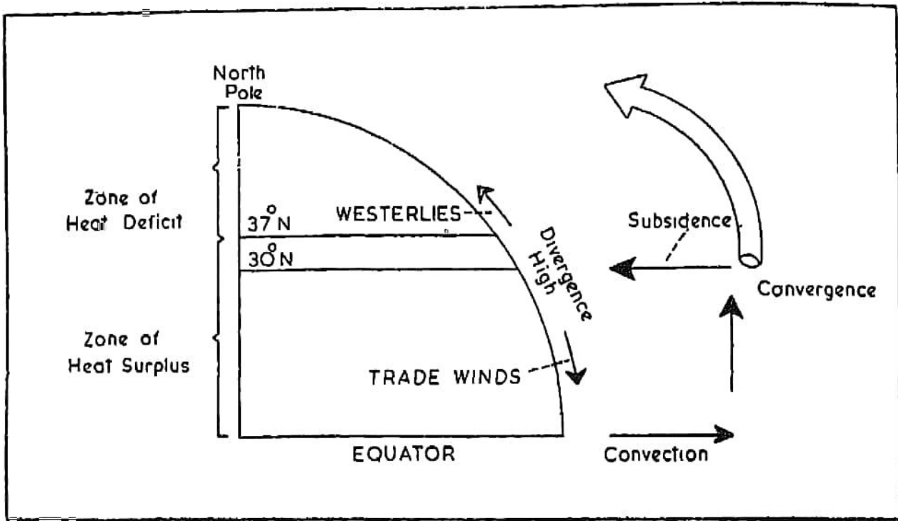
Fig. 75. Formation of a Jet Stream
