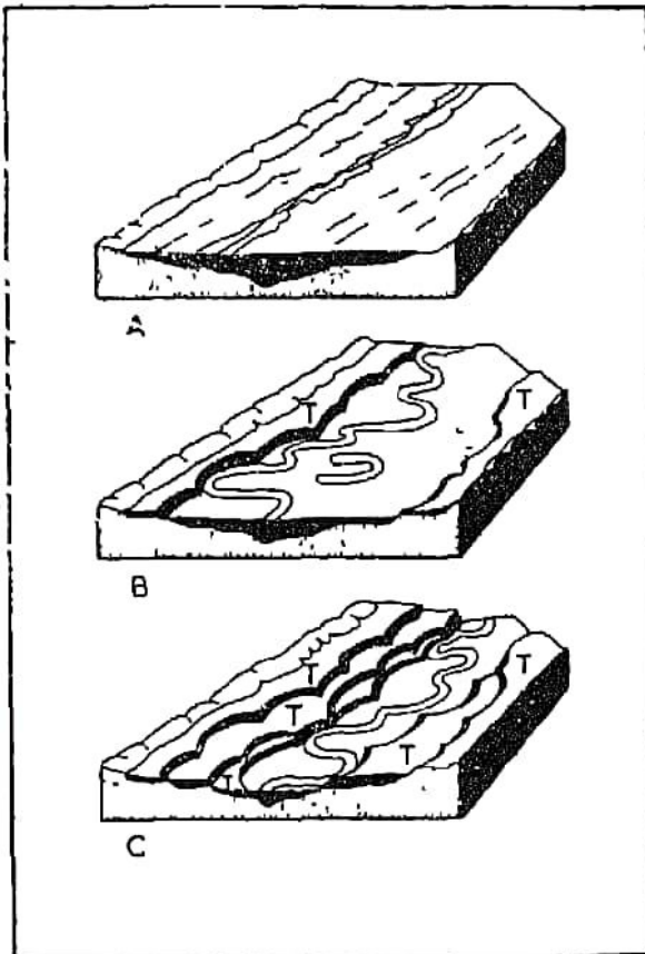
Fig. 34. Alluvial Terraces
