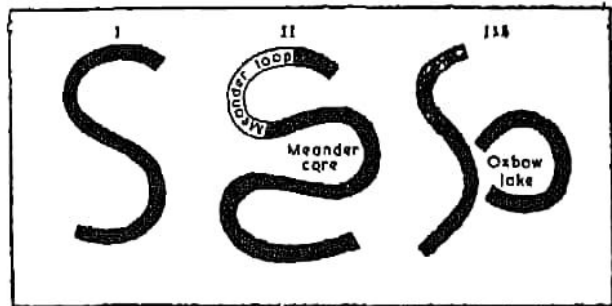
Fig. 32. Stages of Meandering and Formation of Ox-bow Lake
