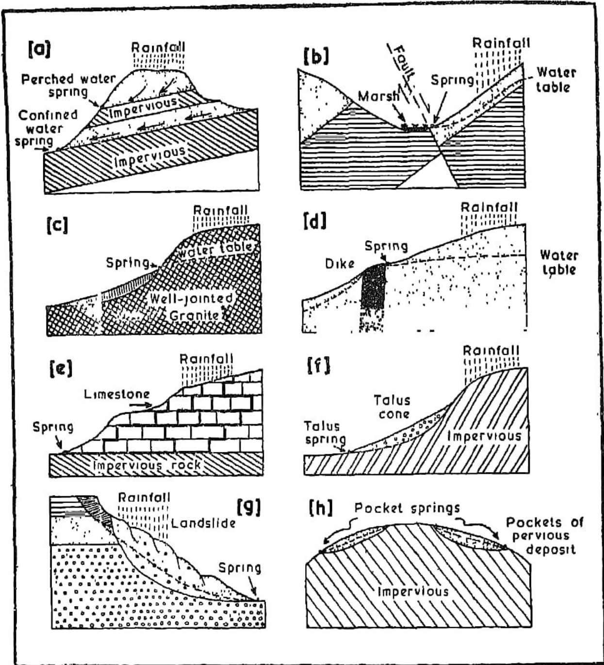
Fig. 91. Formation of Springs
