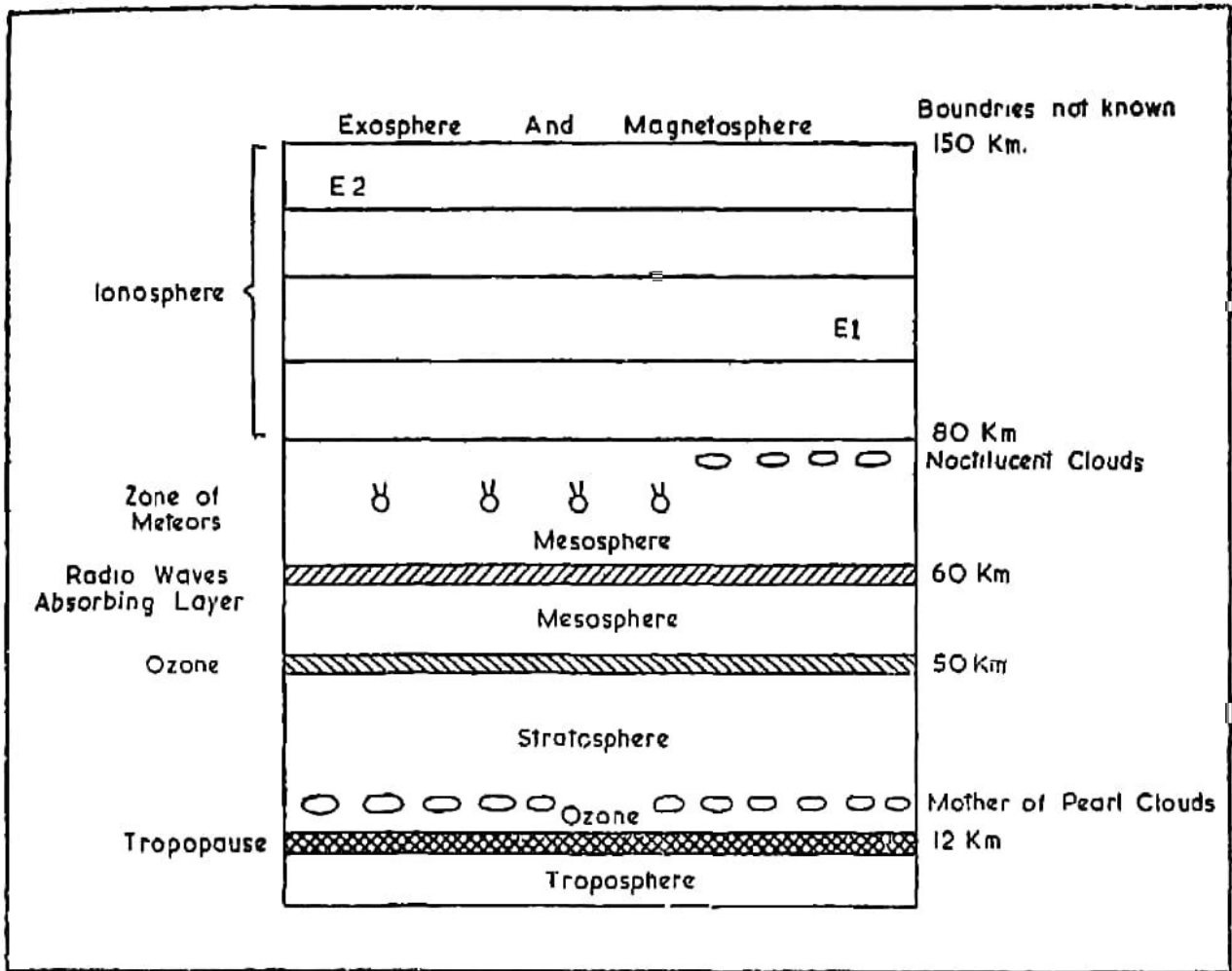
Fig. 56. Layered structure of Atmosphere
