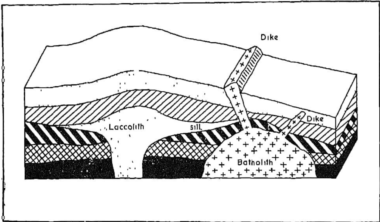
Fig. 15. Four types of Intrusive Rock Masses
