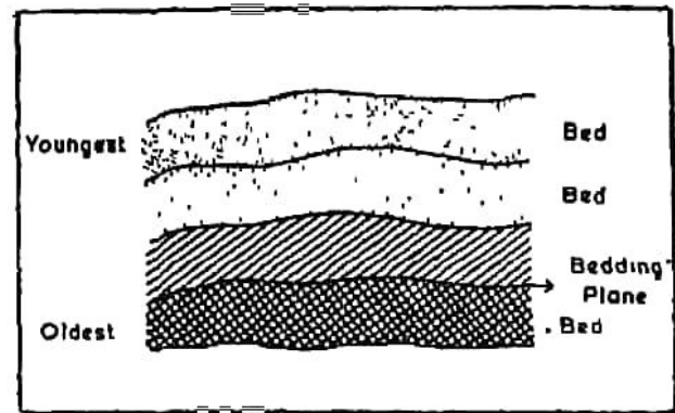
Fig. 17. Sedimentary rock
