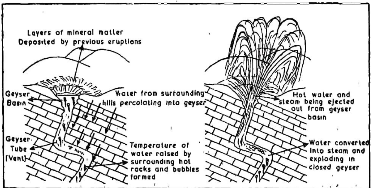
Fig. 94. Formation of Geyser
