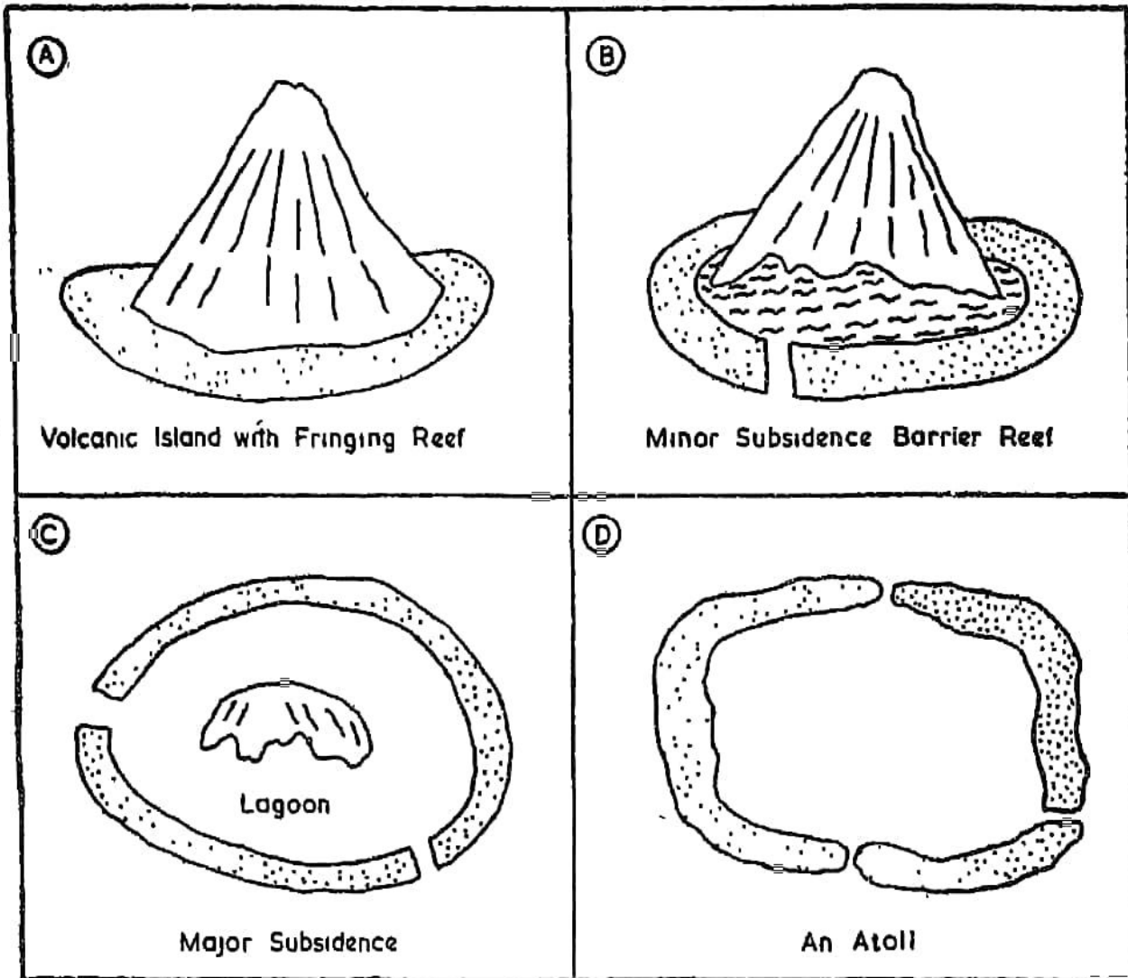
Fig. 112. Types of Reefs
