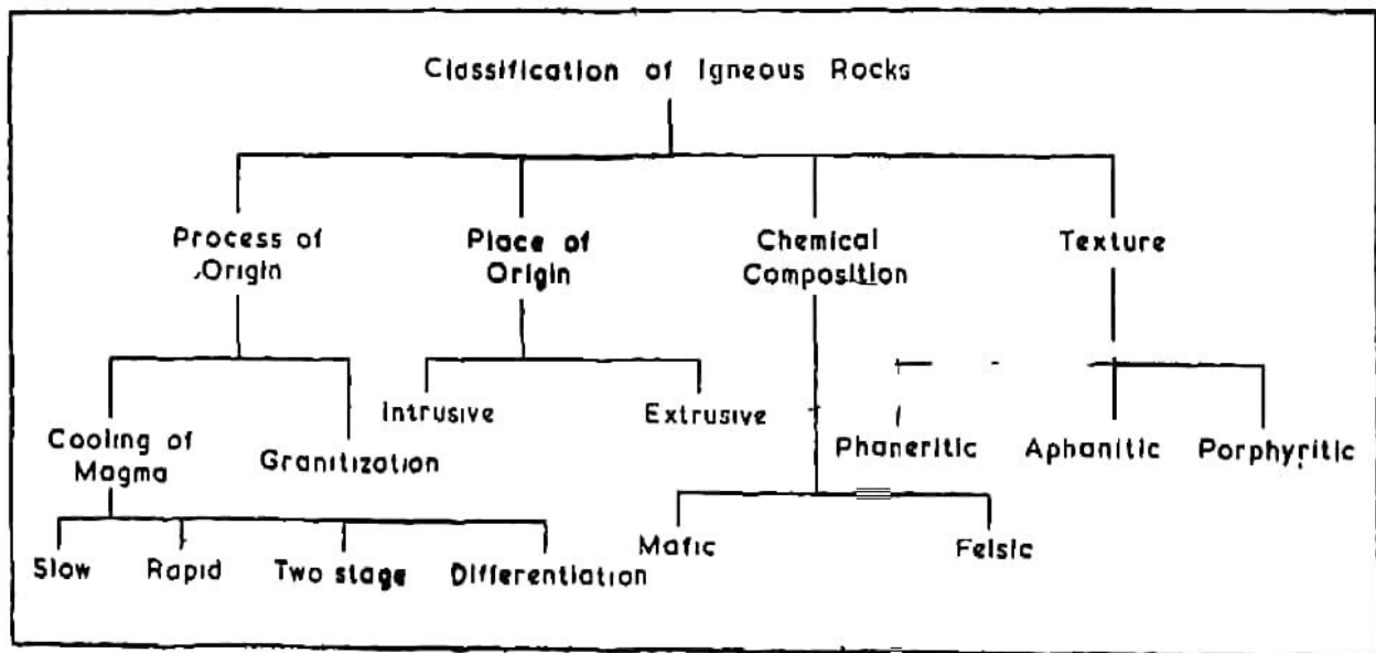
Fig. 16. Classification of Igneous Rocks
