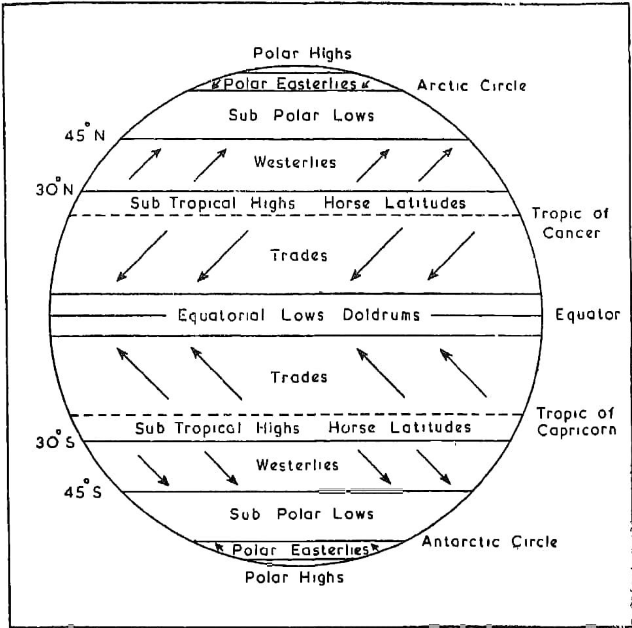
Fig. 70. Planetary Winds
