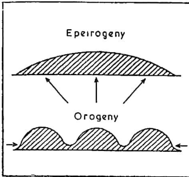
Fig. 44. Epeirogeny and Orogeny
